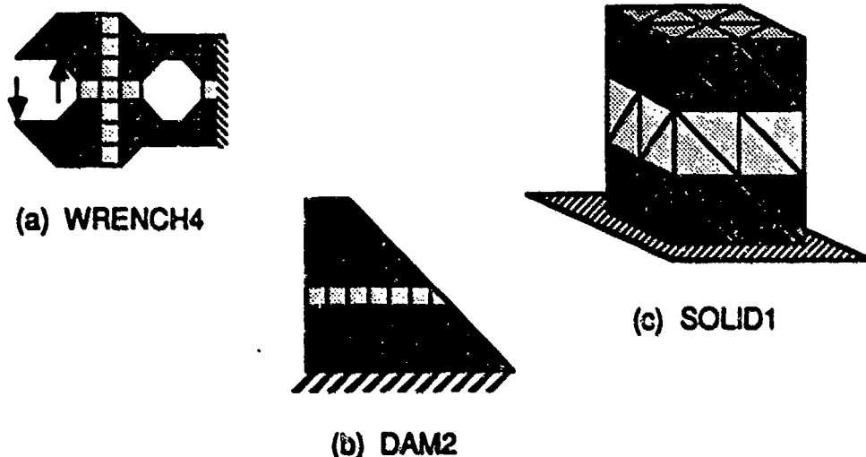
Figure 6.1: Models for Small Full-Rank Problems
