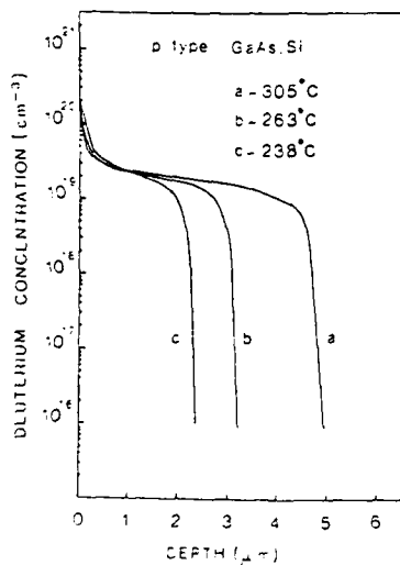
Fig. 1 - D concentration profiles in p + type GaAs: Si (p=10 19 cm -3 ) exposed to R.F. D plasma for 90 min.
