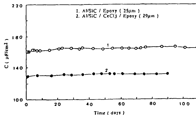
Fig.42 Time dependence of the capacitance C_c for Al/SiC with a 25 \mu\text{m} epoxy coating (curve 1) and Al/SiC which had been pretreated by immersion in \text{CeCl}_3 and coated with a 29- \mu\text{m} epoxy coating (curve 2) during exposure to 0.5 N NaCl.
