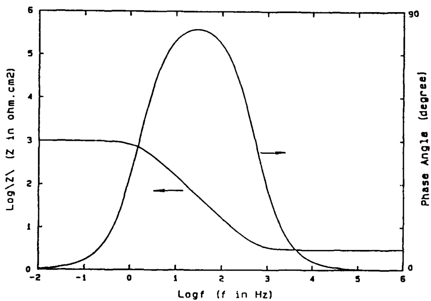
Fig.3.b Bode-plots for the OTCM. R_s = 3 \text{ ohm} , R_p = 10^3 \text{ ohm} , C = 10^{-4} \text{ F} , and A = 1 \text{ cm}^2 .
