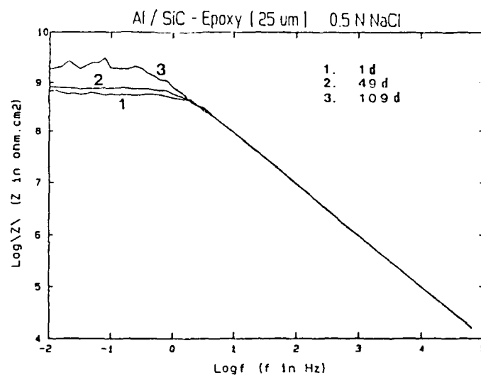
Fig.41 Bode-plots for Al/SiC with a 25- \mu\text{m} epoxy coating as a function of exposure time to 0.5 N NaCl.
