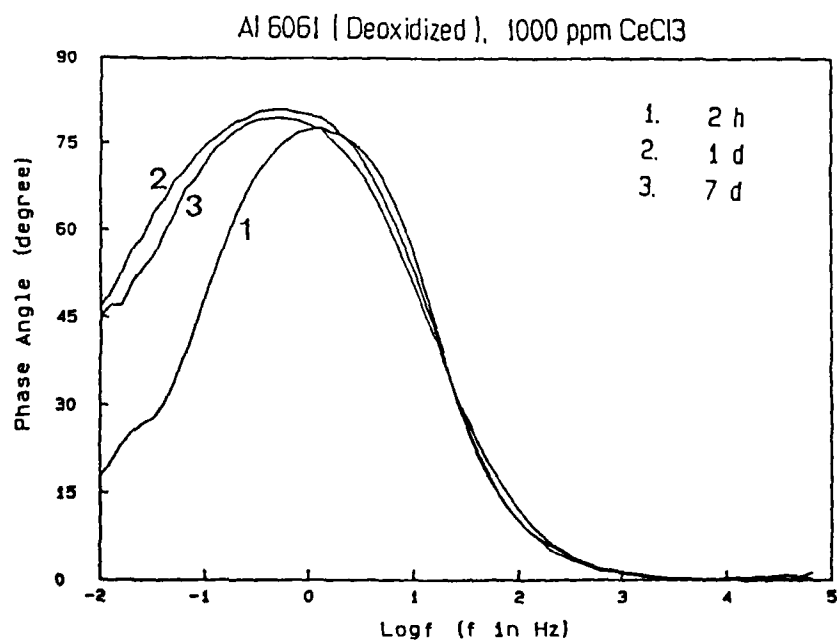
Fig.19.a and b Bode-plots for deoxidized Al 6061 as a function of immersion time in 1000 ppm \text{CeCl}_3 .
