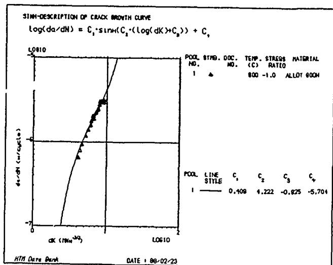
Fig. 8. Sinh-Description of a Crack Growth Curve
