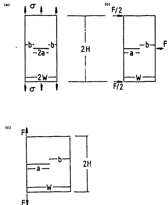
Figure 2. The specimen geometries that were analysed. (a) CCT, (b) SECB, (c) CT.
