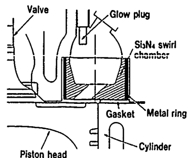
Fig.7 Mounting and assembly of a silicon nitride precombustion (swirl) chamber [6].
