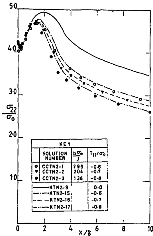
Figures 6. Variation of stress directly ahead of the notch tip for the CCT specimen with a/W = 0.5 , H/W = 2 . LEFT - n = 0.2 . RIGHT - non-hardening.
