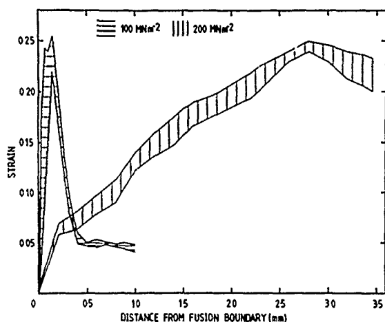
Fig. 6 Variation of local strain in weld testpieces for tests undertaken at 100 MPa and 200 MPa at 838K. In each case, fracture occurred near the point of maximum strain.
