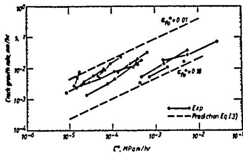
Fig. 3 Crack growth rates as a function of C^* , for normalised and tempered 1/2 CrMoV (from Neale[8])
