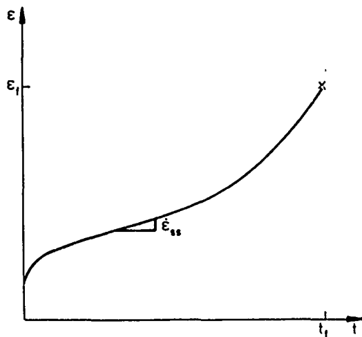
Fig. 1. A typical creep curve obtained from a uniaxisal test at constant stress.
