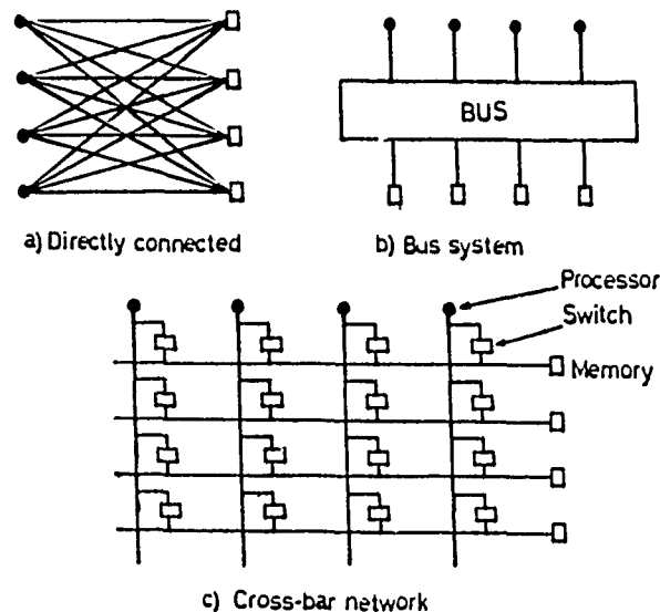
FIG1-SHARED MEMORY SYSTEMS
