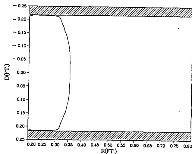
M=2.50 CONTOUR 47%NSR Long Duct Solution
