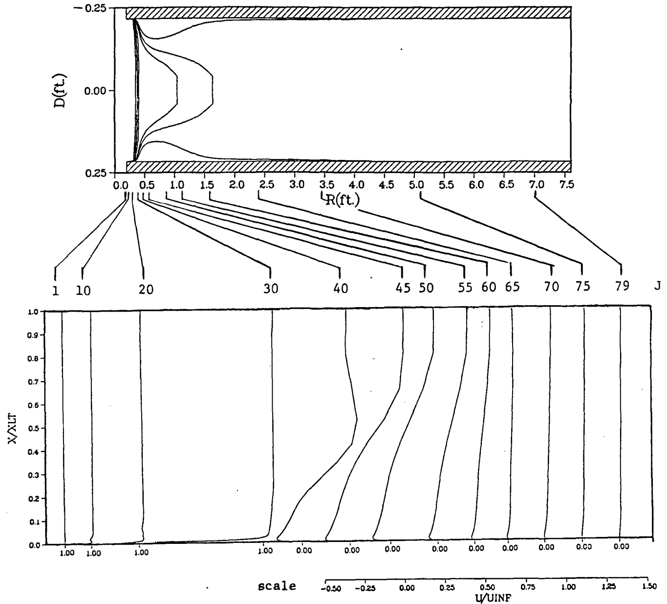
Figure 56. Velocity Profiles, Case 3b Converged Solution.
