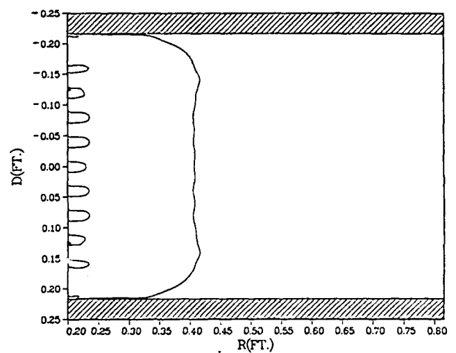
M=2.5 CONTOUR 47%NSR Actual Inflow Solution
