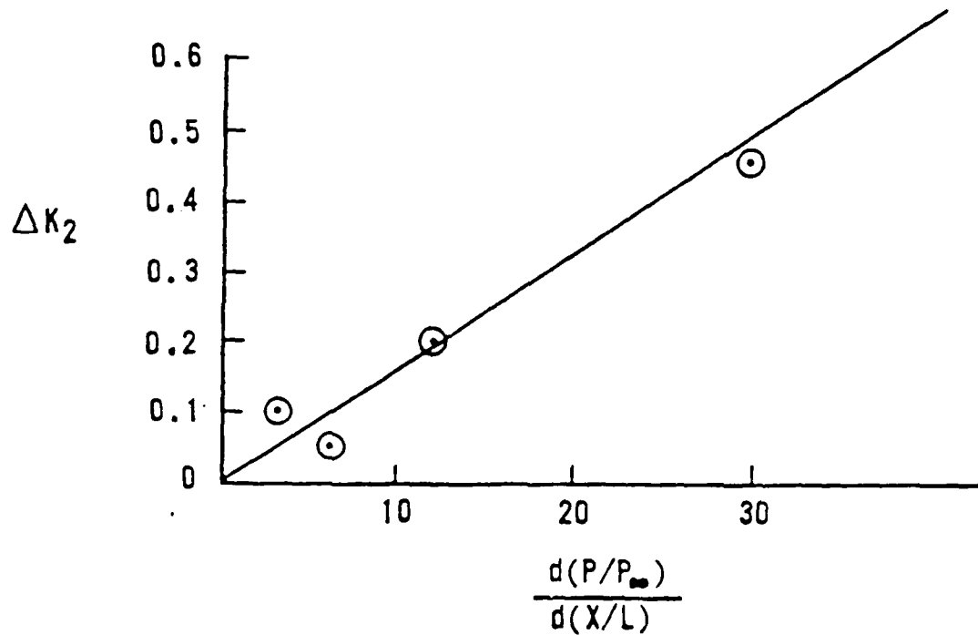
Figure 16. Variation in Clauser's Constant ( k_2 ) With Nondimensionalized Adverse Pressure Gradient. Experimental data of Laderman (69), Sturek (70), and Waltrup and Schetz (71).
