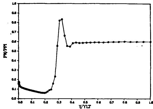
N=125K PW/PPI CSM 60%NSR WBB=2
