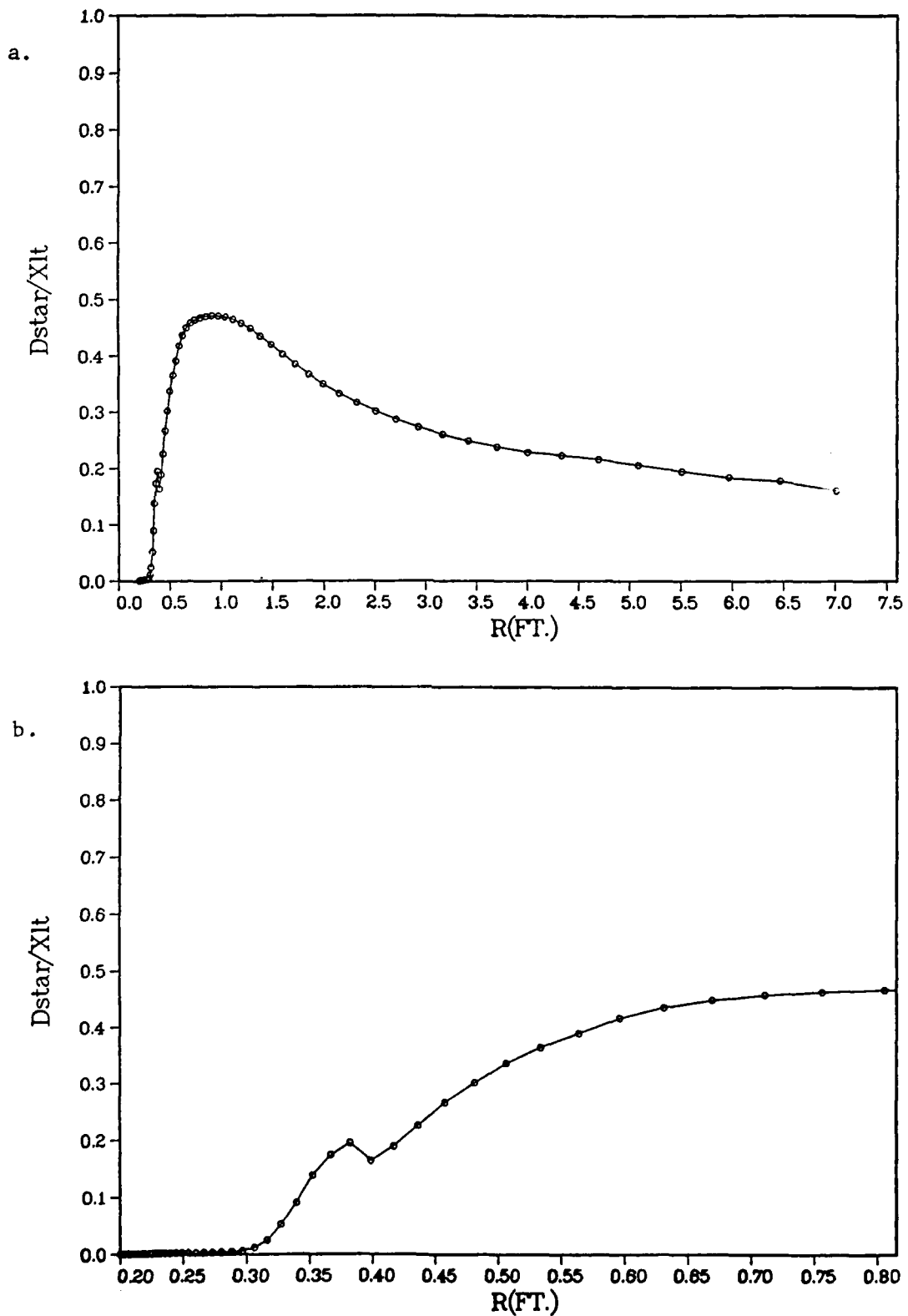
Figure 60. Plot of Case 3b Converged Solution Kinematic Displacement Thickness; a) Full Diffuser Length; b) Length Corresponding to Baseline Diffuser.
