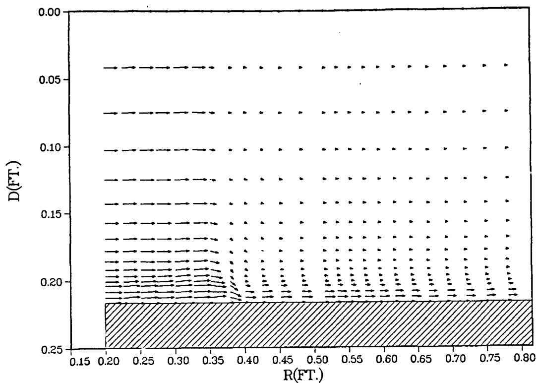
Figure 31. Velocity Vector Plot, Case 2b Converged Solution.
