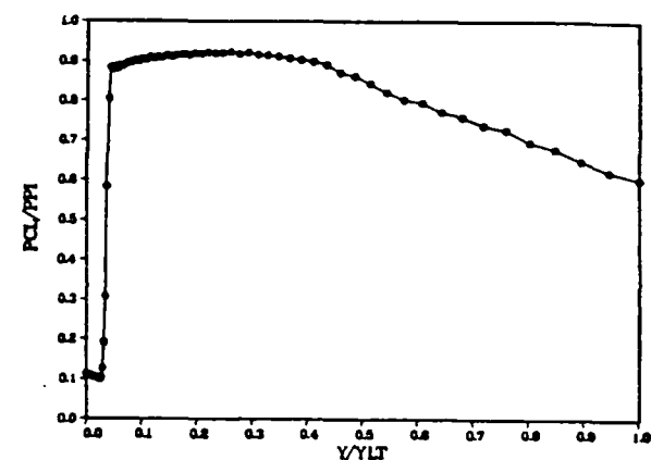
N=100K PCL/PPI CSB 60%NSR WBB=2
