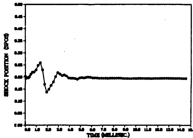
CONVERGENCE TIME HISTORY 60%NSR
