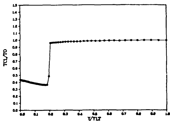
N=1 TCL/TO CSM 60%NSR WBB=2
