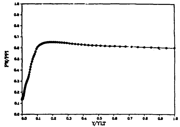
N=75K PW/PPI CSM 60%NSR WBB=0
