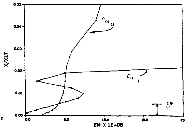
PLOT OF EMI AND EMO 60% NSR SOLUTION (J=30)
