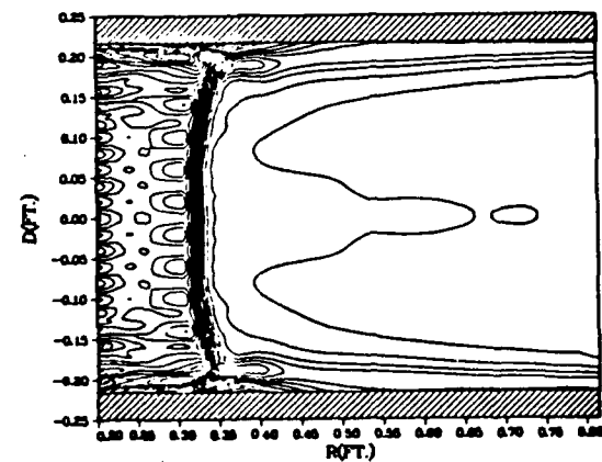
N=110K ACTUAL INFLOW 60%NSR WBB=.195
