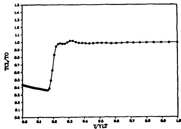
N=10K TCL/TO CSB 60%NSR WBB=0
