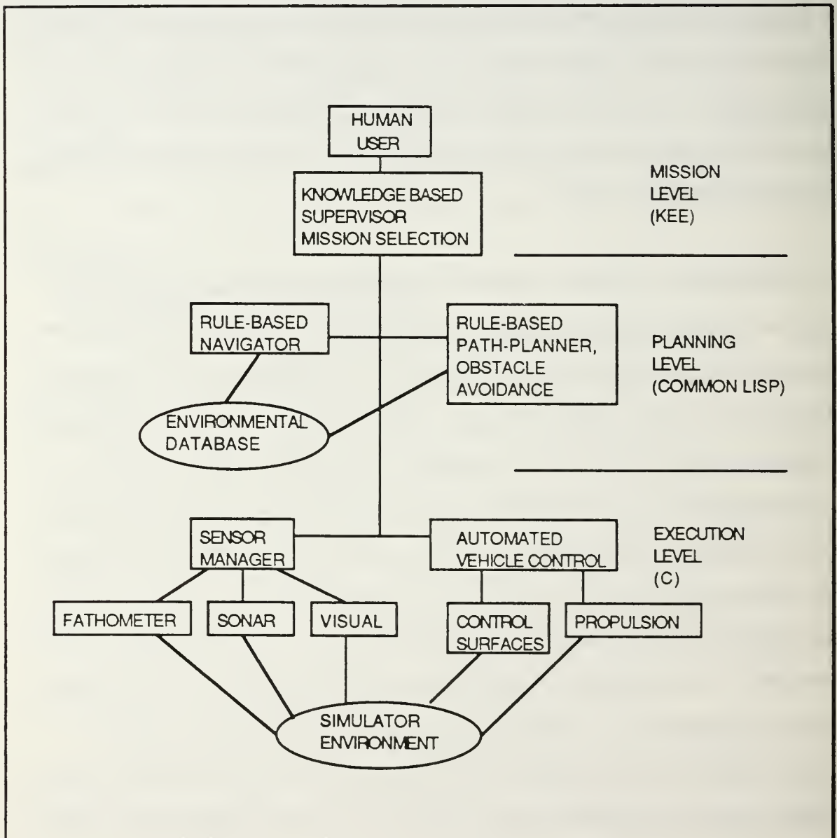
Figure 4.1 Hierarchical System Architecture
