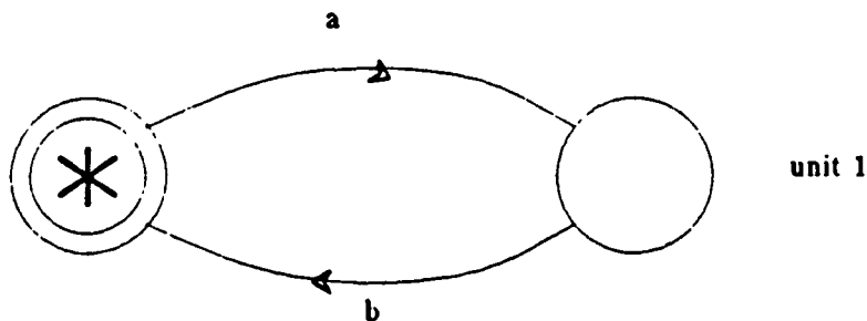
Figure 4.5: A unit machine for (ab)^o
