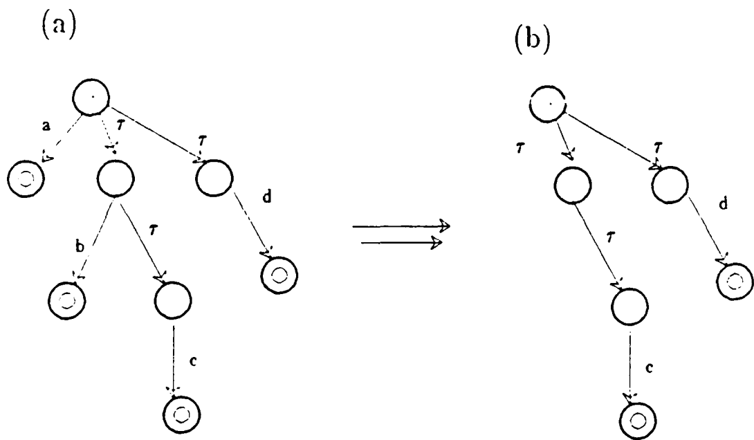
Figure 6.5: Equivalent Structures for minL
