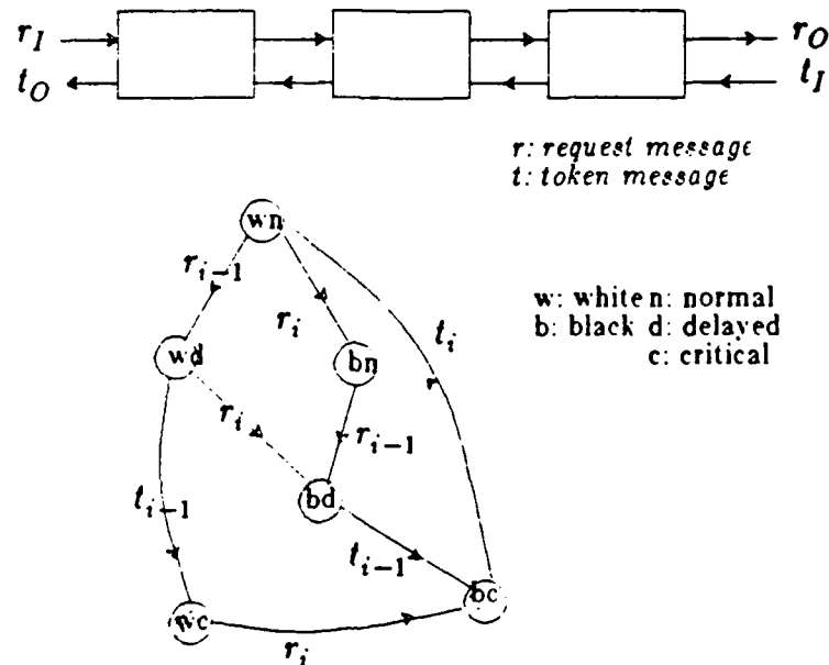
Figure 7.11: Mutual Exclusion in a Ring
