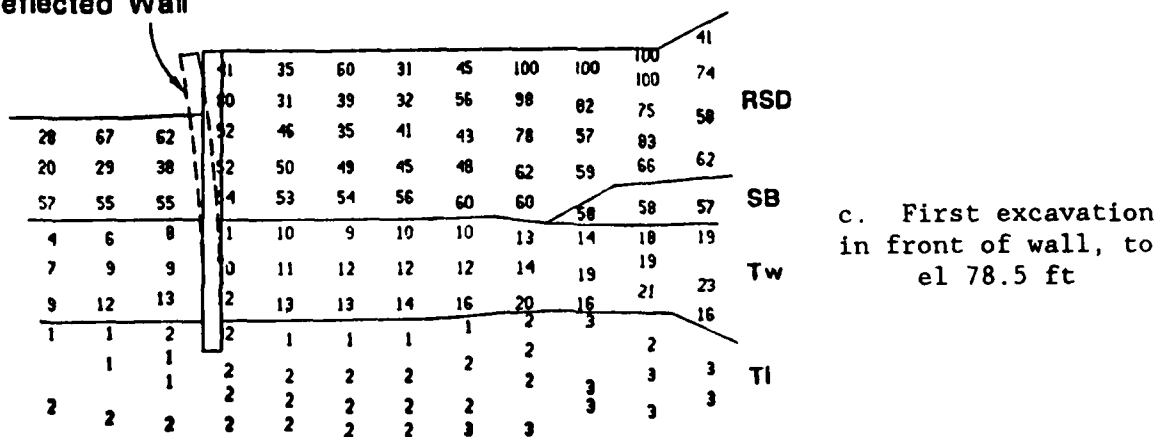
Figure 9. Percent of mobilized shear strength during construction operations at Panel 6
