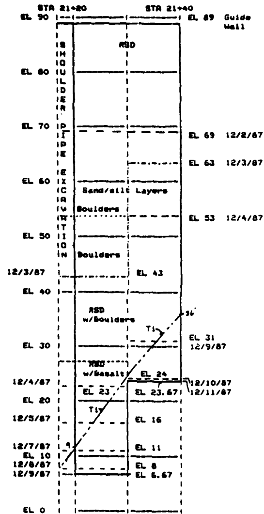
Figure 46. Panel 11, as-constructed
