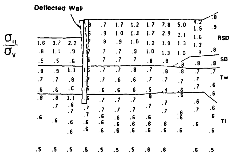
c. First excavation in front of wall, to el 78.5 ft
