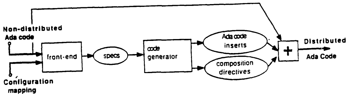
Fig.5 DTK architecture
