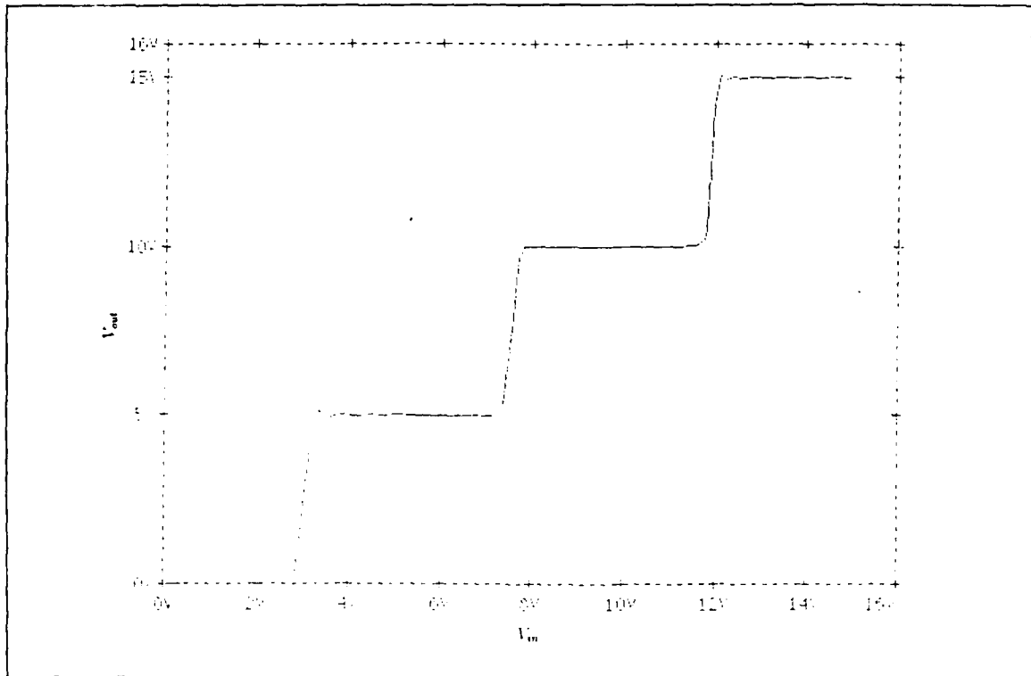
Figure 5.7: Latch Input/Output DC Characteristics ( V_{dd} = 15\text{ V} )
