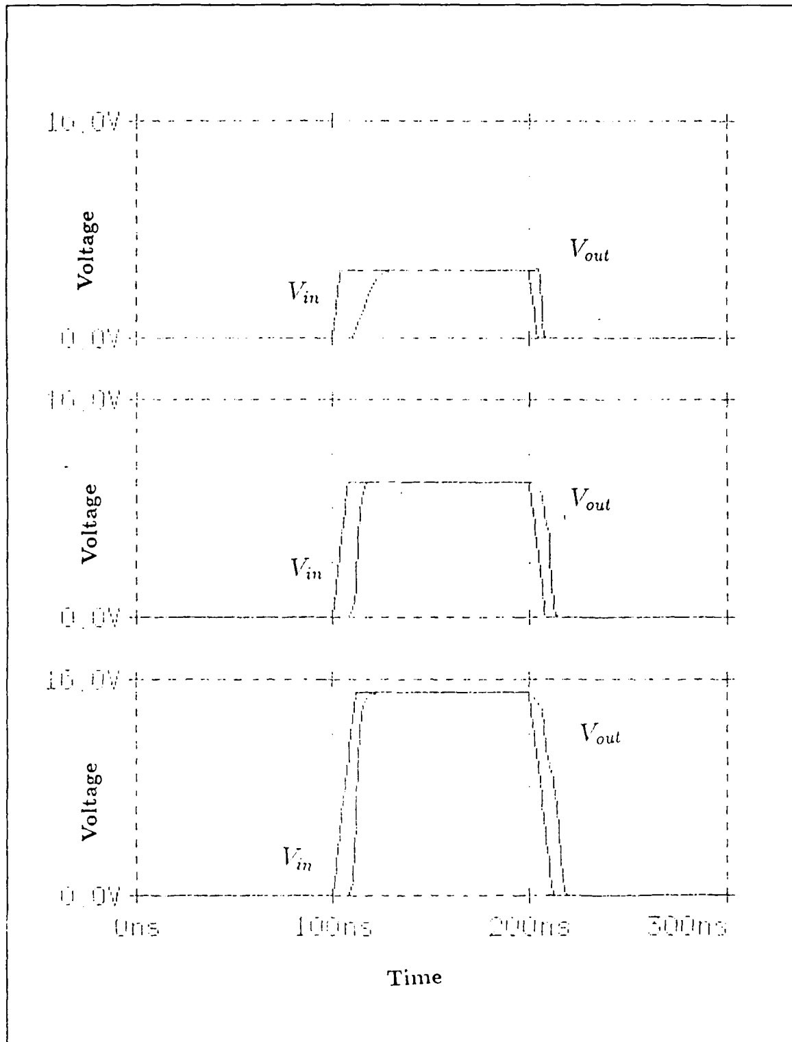
Figure 5.8: Latch Response to Step Inputs ( V_{dd} = 15\text{ V} )
