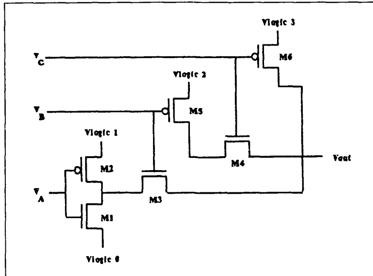
Figure 5.4: CMOS Realization of a Four-Valued Voltage Encoder
