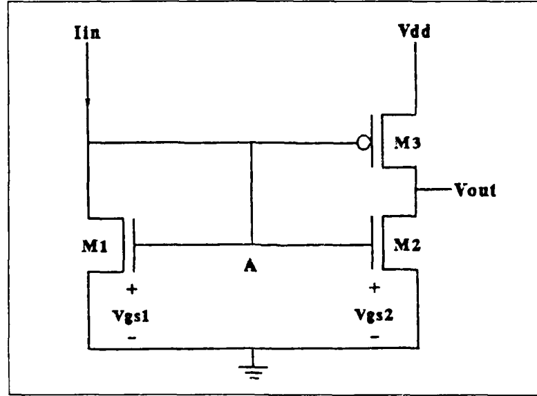
Figure 2.4: Current-Controlled CMOS Inverter
