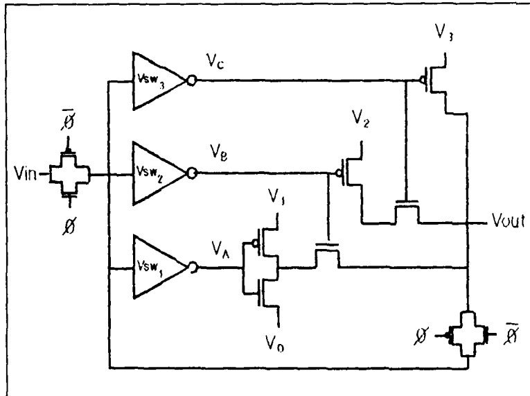
Figure 5.5: Four-Valued Voltage-Mode CMOS Data Latch
