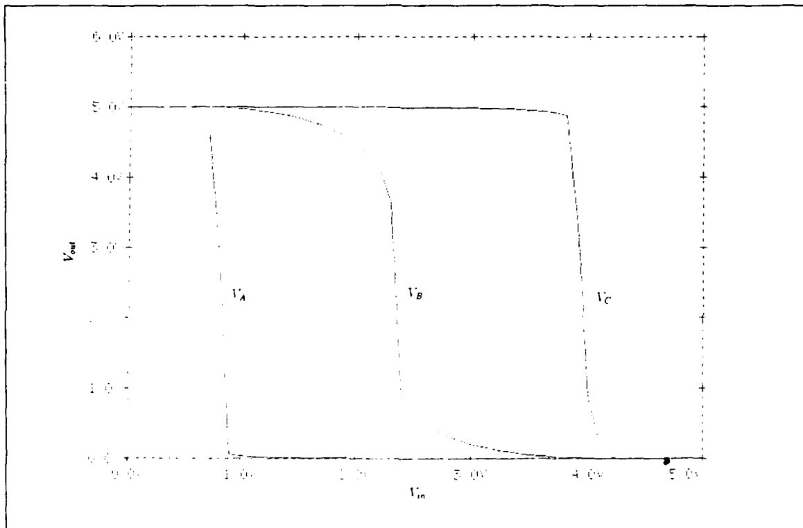
Figure 5.11: Threshold Detector DC Characteristics ( V_{dd} = 5 \text{ V} )
