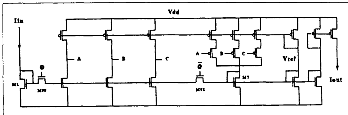
Figure 4.3: Modified Current-Mode CMOS Four-Valued Data Latch
