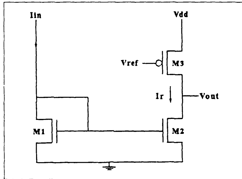
Figure 2.5: CMOS Current Comparator (After Ref. 13)
