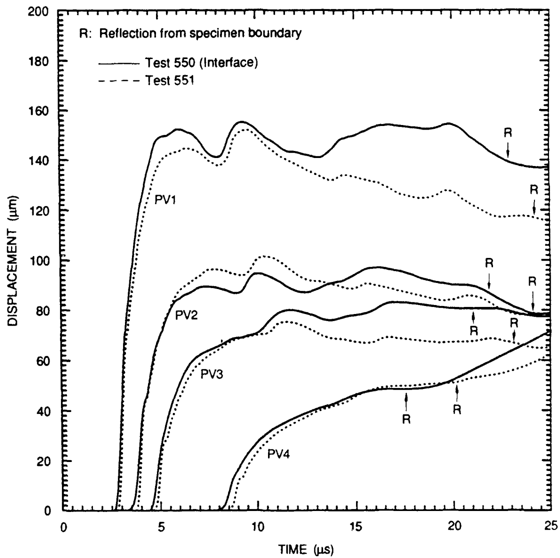
Figure 7. Displacement histories in Sierra White granite (Tests 550 & 551).
