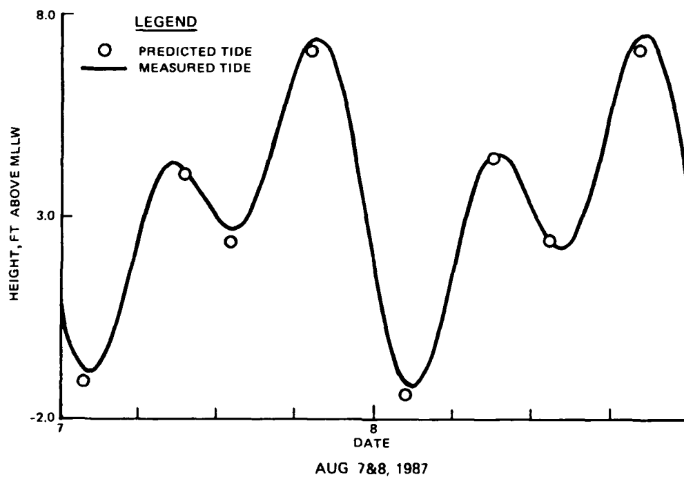
Figure 11. Predicted tide versus measured tide 7 and 8 August 1988
