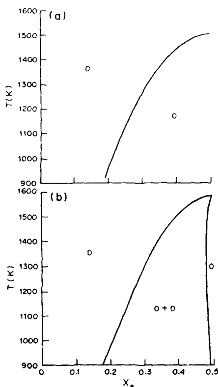
Fig. 4. Calculated phase diagram for solid phases only for (a) Case I and (b) Case II. Diagram is symmetric about x_B = 0.5 . D and O represent the disordered and ordered phases respectively.
