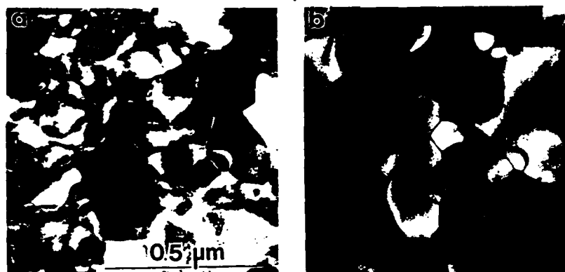
FIG.3 TEM bright-field (a) and dark-field (b) of #4 alloy cooled from 1400°C. Dark-field shows only one (out of four rotational domains of the omega-type phase. Interfaces within the domains separate translational domains.
