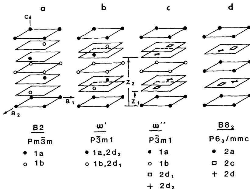
Fig. 1. Schematic drawing of (a) B2; (b) hypothetical \omega' ; (c) \omega'' ; (d) B8 2 crystal structures. Different symbols represent different sites occupancies.
