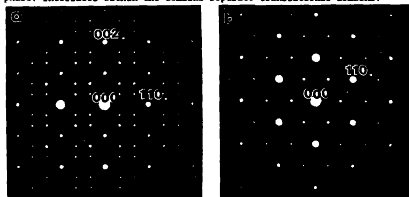
FIG.4 SADP patterns typical for the alloy #4 cooled from either 1400°C or 1100°C. a) [110]_{bcc} zone axis; b) [111]_{bcc} zone axis.
