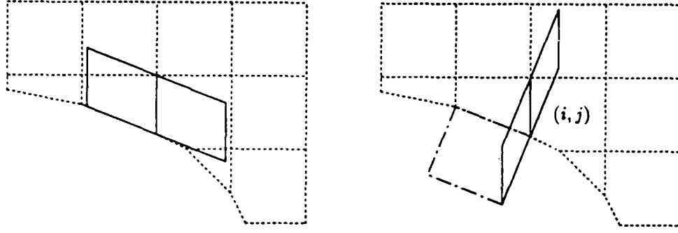
Figure 5: (a) Tangential boxes constructed from the cell interface. (b) Normal boxes from the cell interface and \text{outbox}(i-1, j) .
