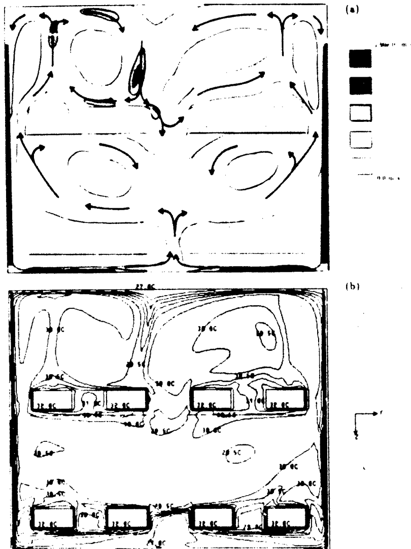
Fig. 2.4 Two-dimensional numerical results at time t=t_o+30s (a) chamber velocity direction and magnitude profile (b) temperature contour
