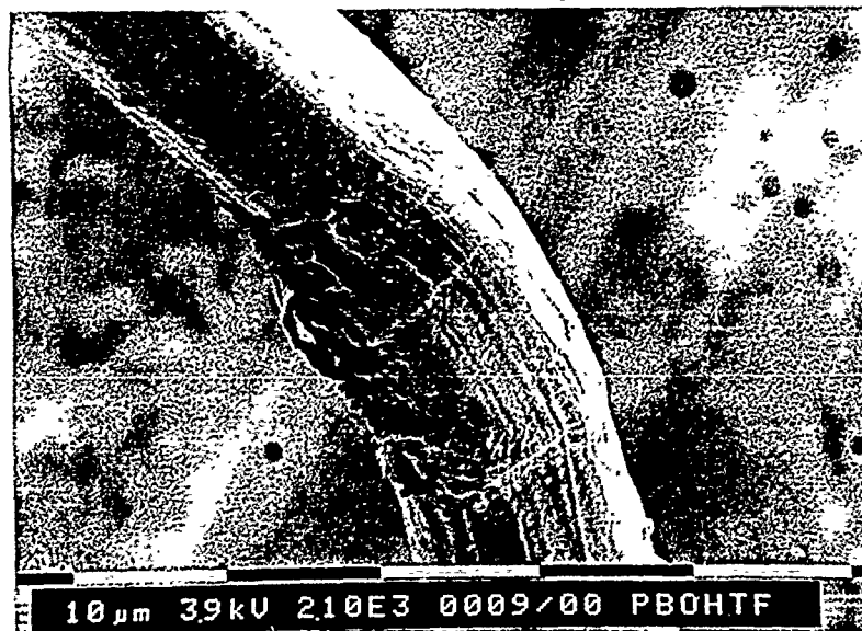
Figure 3.20(b) Tensile recoil damage observed in HT PBO fibre.
