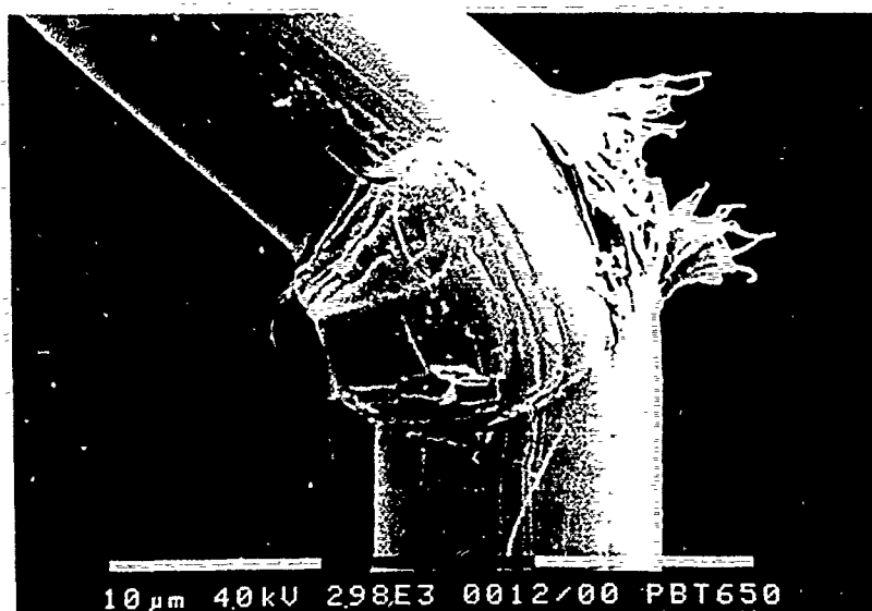
Figure 3.59(b) Kinkbands caused by bending in HT PBT fibre.
