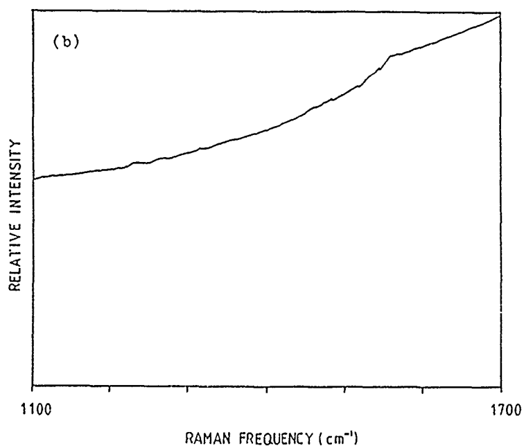
Figure 3.33 Raman spectra in the range of 1100\text{--}1700\text{ cm}^{-1} for individual ABPBO fibres obtained at 0% fibre strain. (a) As-spun; (b) heat treated
