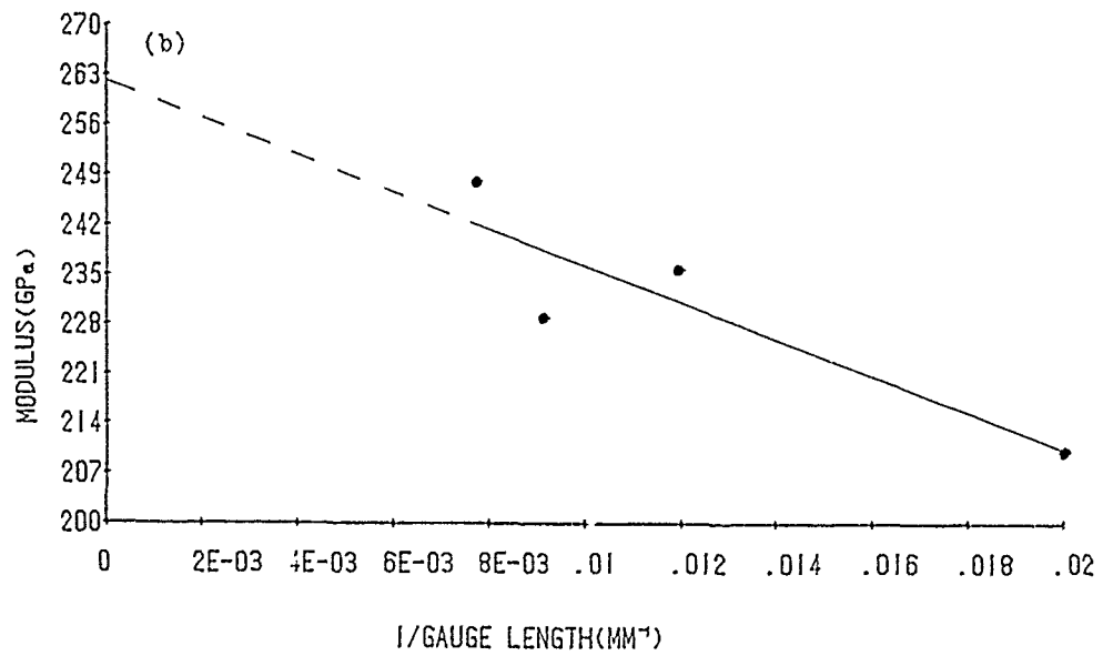
Figure 3.23 Young's modulus versus 1/\text{gauge length} curves for PBO fibres. (a) As-spun; (b) heat treated
