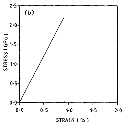
Figure 3.10 Stress-strain curves for individual PBT fibres.
