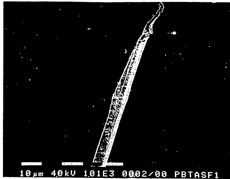
Figure 3.15(a) SEM of AS PBT fibre fracture surfaces.
