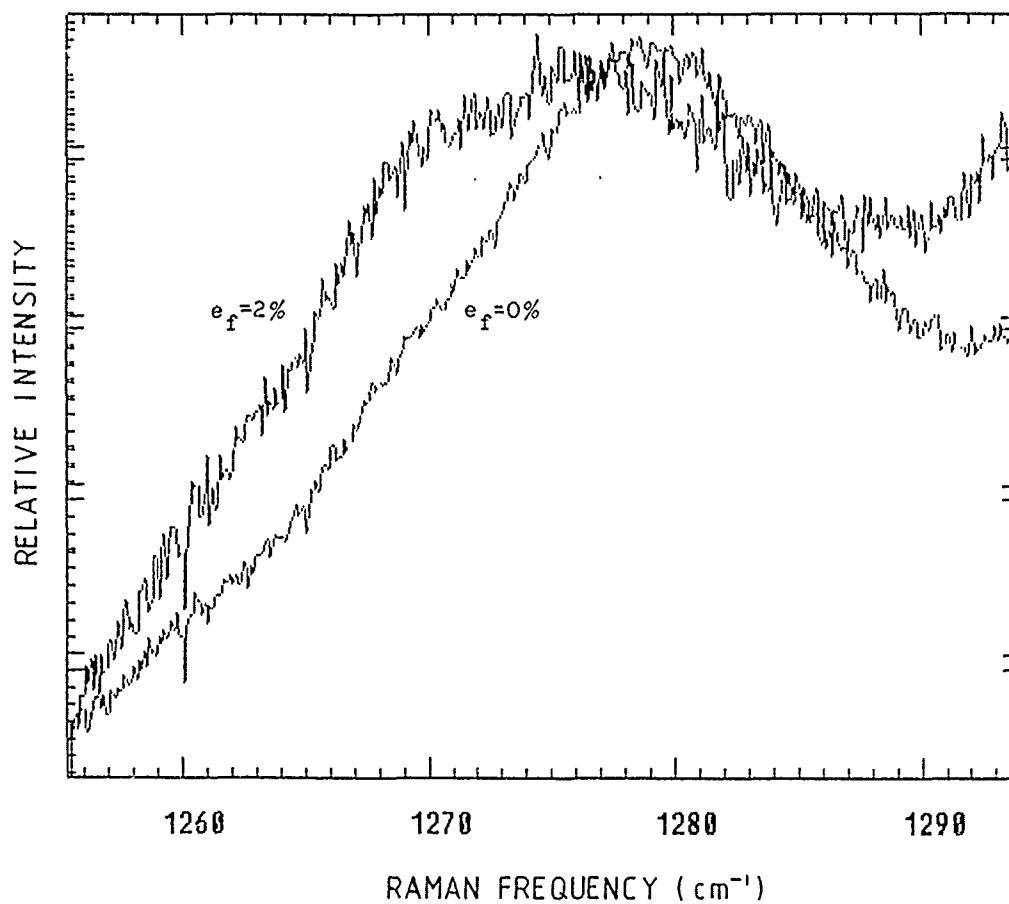
Figure 3.37(a) Raman spectra in the region of the 1275 cm -1 band for an AS PBO fibre obtained at fibre strain ( e_f ) of 0% and 2% showing the peak shift using He/Ne laser.
