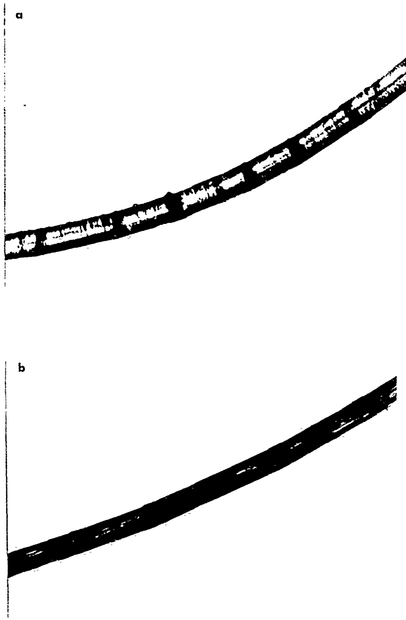
Figure 3.63 Optical micrographs of as-received PBO fibres deformed by bending in air. (a) As-spun; (b) heat treated
