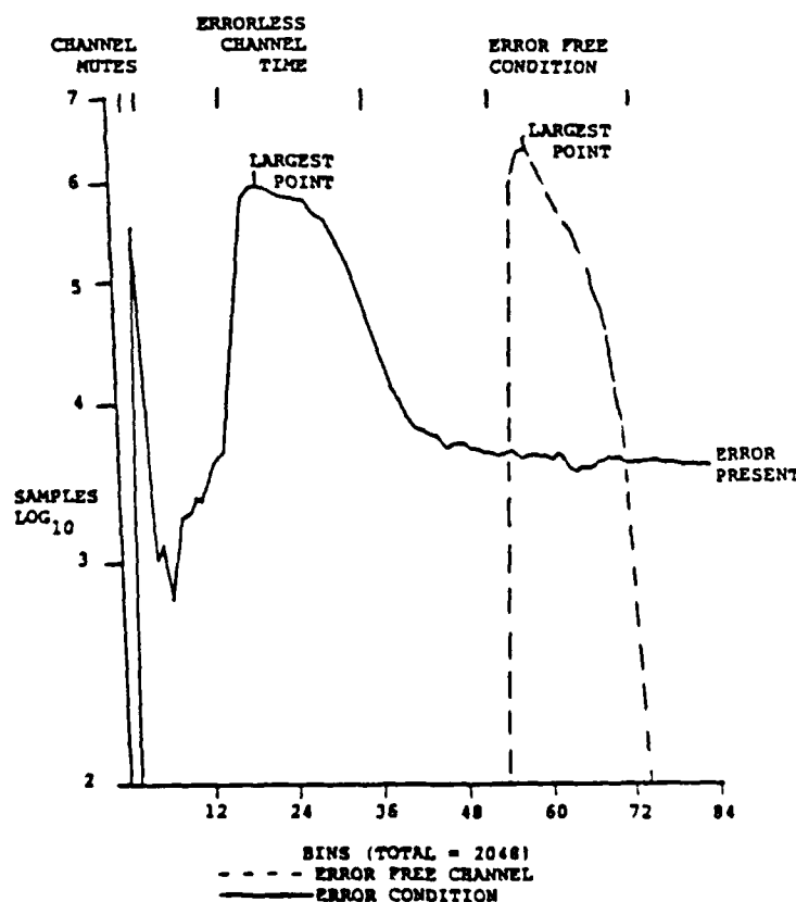
Figure 6.2 Energy Histogram
