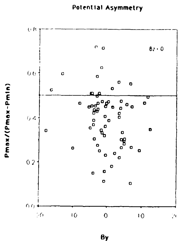
Figure 4. Dependence of Potential Asymmetry on IMF B_y .
