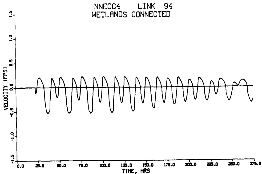
Figure J30. Average channel velocities in EGG-WFCC under non-navigable entrance, no by-pass connector channel to marina conditions
