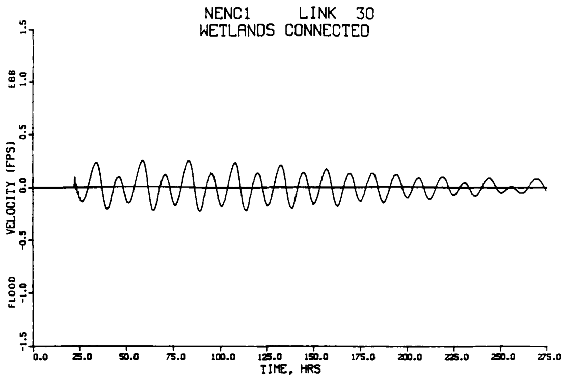
Figure D21. Average channel velocities in Huntington Harbour under navigable entrance, navigable connector conditions
