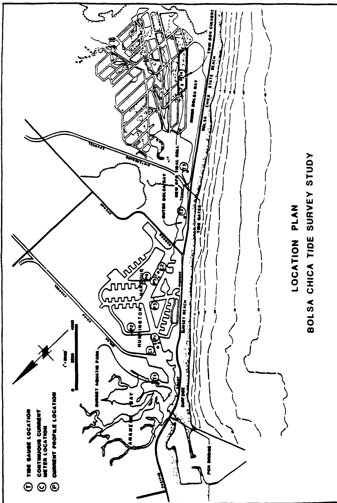
Figure 13. Location of prototype field survey tide gages and velocity meters (after Moffatt & Nichol, Engineers 1986)
