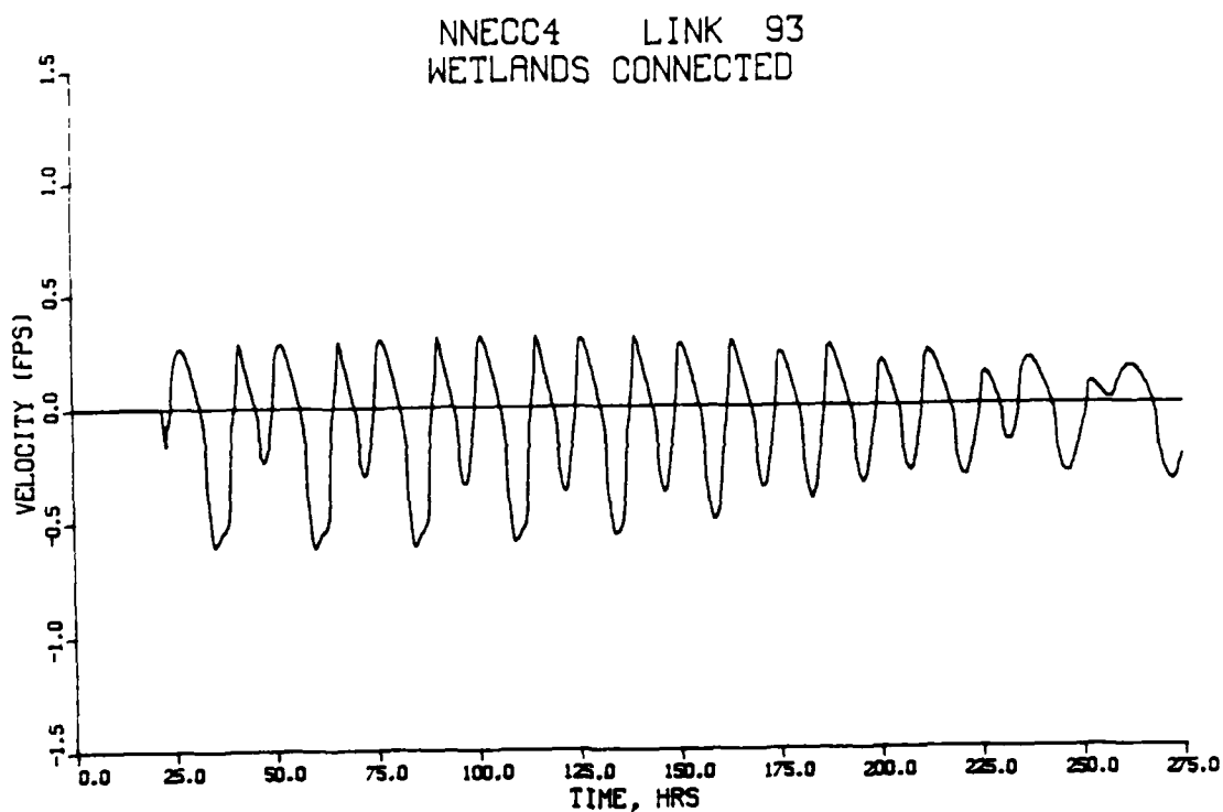
Figure J29. Average channel velocities in EGG-WFCC under non-navigable entrance, no by-pass connector channel to marina conditions
