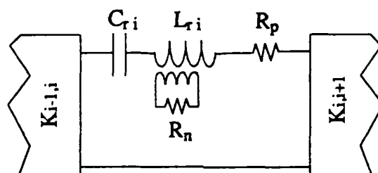
(a) Series active tank.
