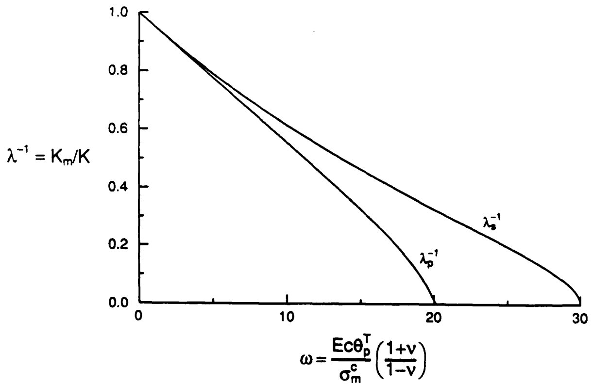
Fig. 2 Reciprocal of peak and steady-state toughening versus \omega , semi-infinite crack.
