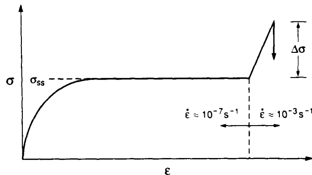
Fig. 3. Schematic stress-strain curve for tests used to evaluate creep damage. The sudden increase in strain rate at a certain level of strain causes the specimen to fracture at an overstress \Delta\sigma .
