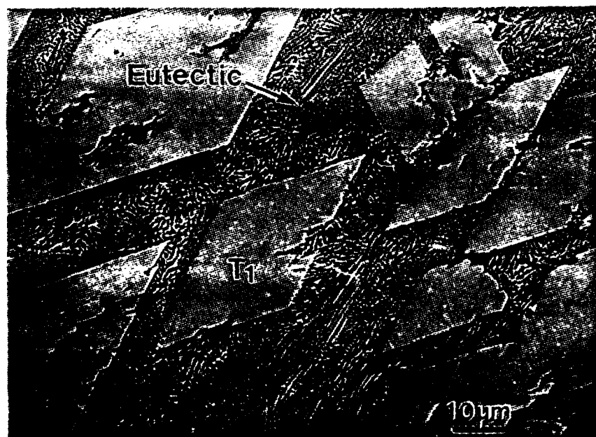
Figure 25: Alloy 12b, \text{Nb}_{45}\text{Si}_{10.4}\text{Al}_{44.6}
