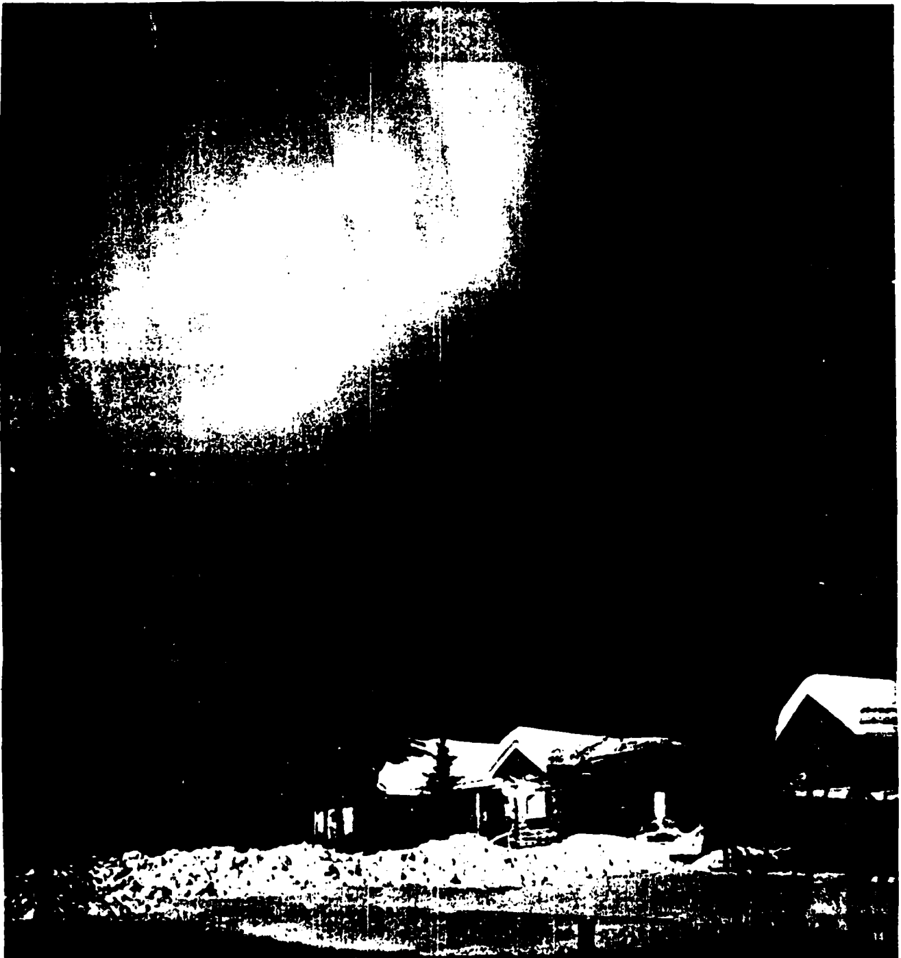
Example of an Aurora Near Fairbanks, Alaska
