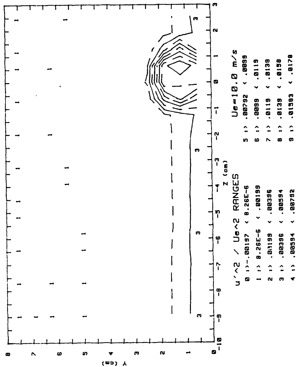
Figure 9. \overline{u'^2} (Boundary Layer, Station A', m = 1.5, \Delta = 0.25 )
