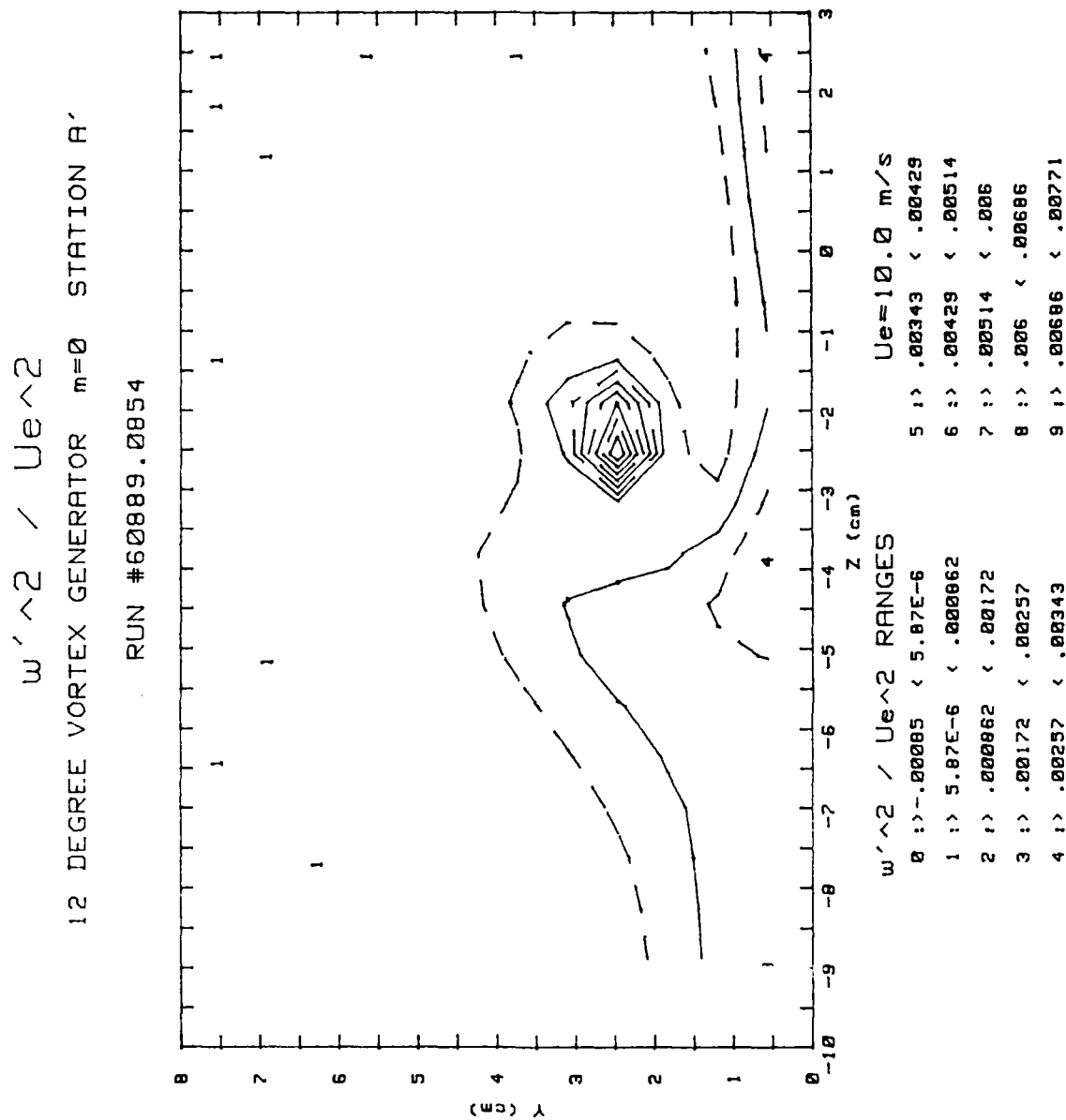
Figure 75. w'^2 (Boundary Layer w/vortex, Downwash @ Centerline, Station A', m = 0 , \Delta = 0.25 )
