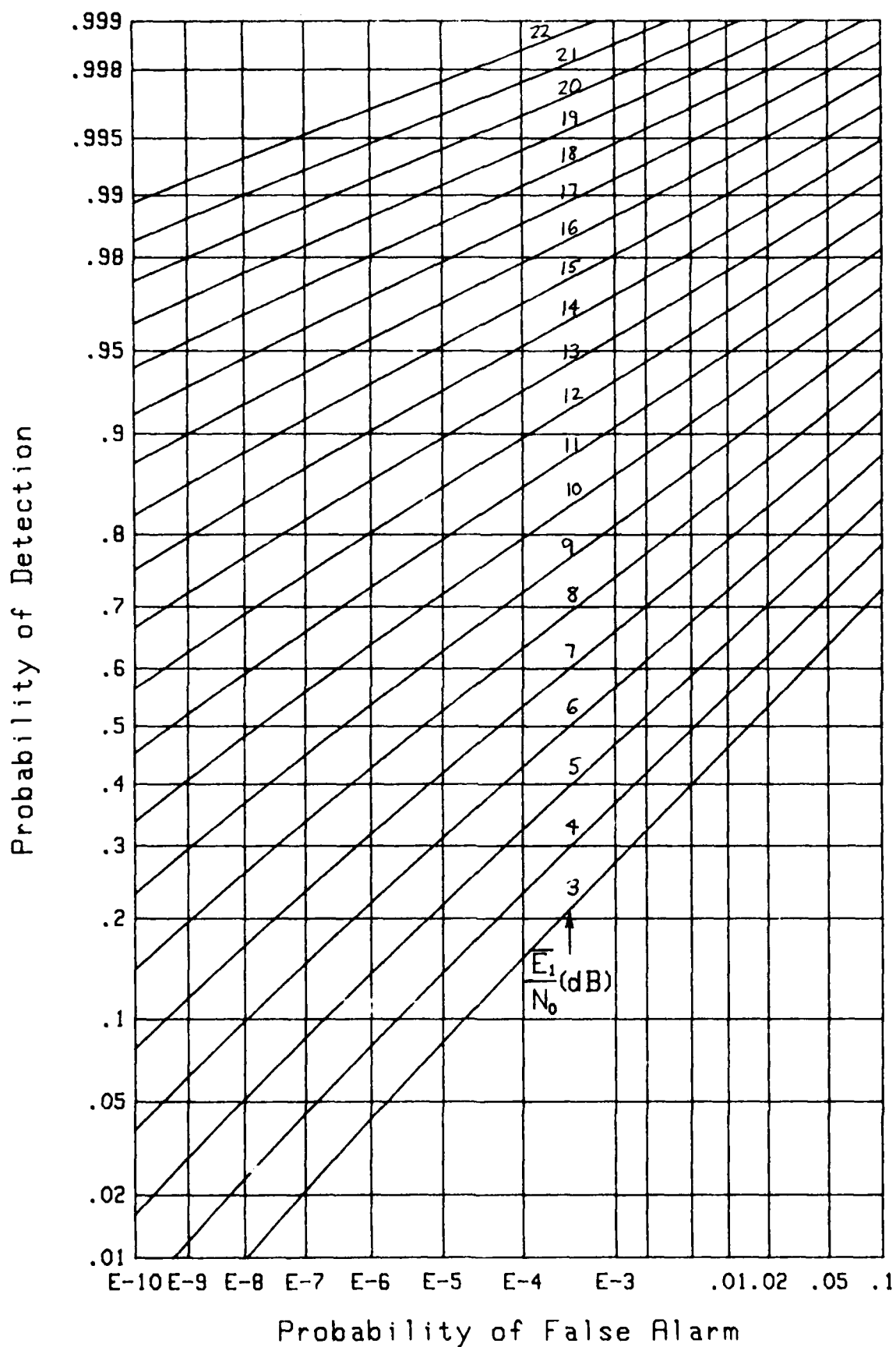
Figure 27. ROC for K=4 , m=.5 , \rho=0 , L=32
