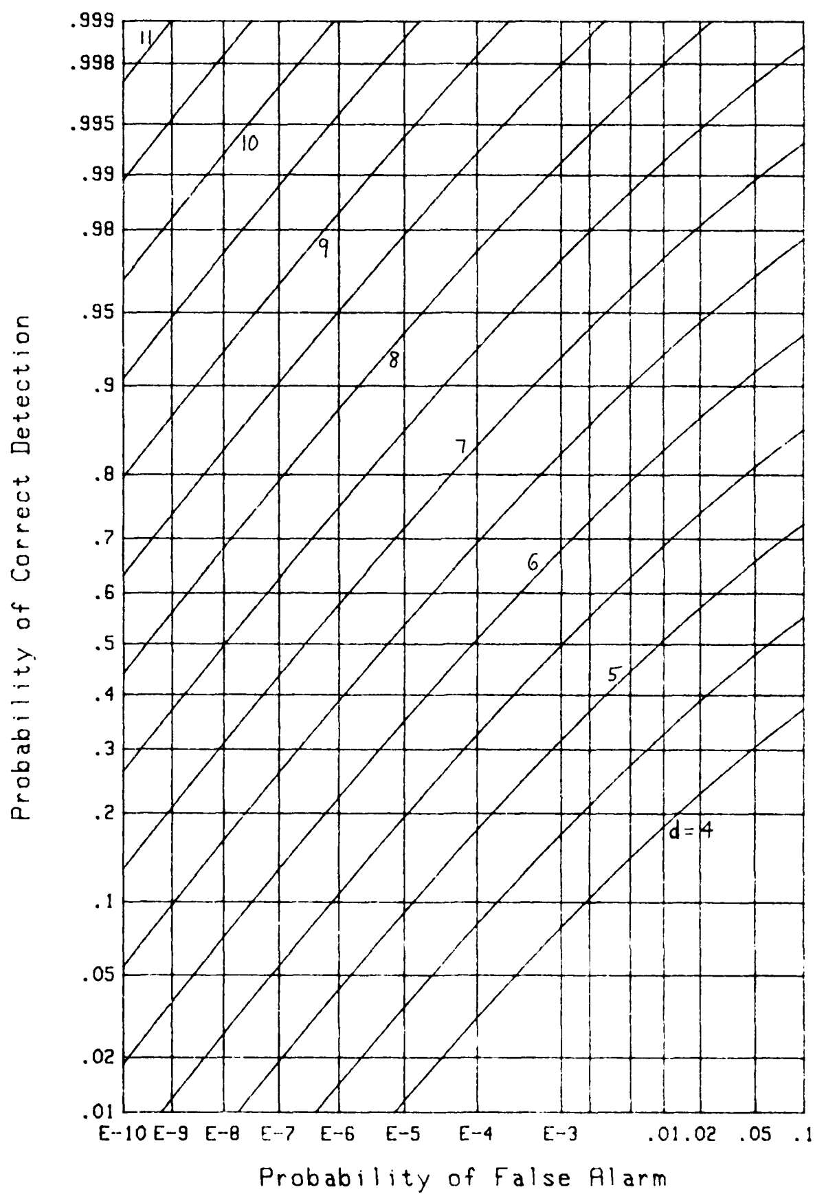
Figure 17. ROC for M=4 , N=100
