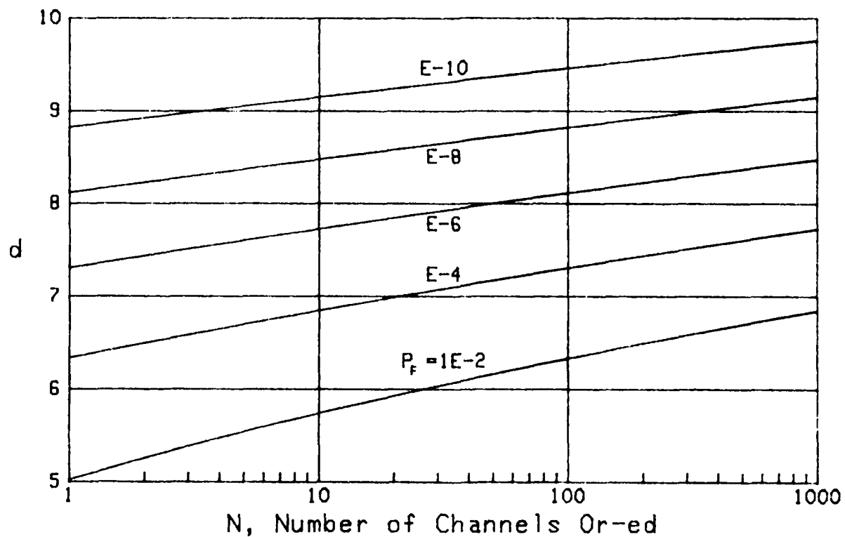
Figure 48. Required d Values for M=4 , P_{c_0}=.9
