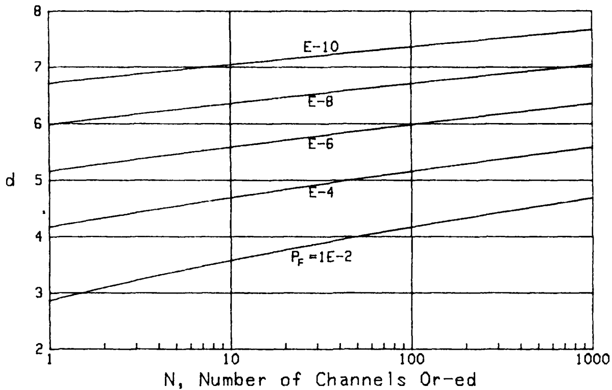
Figure 43. Required d Values for M=1 , P_{cd}=0.5
