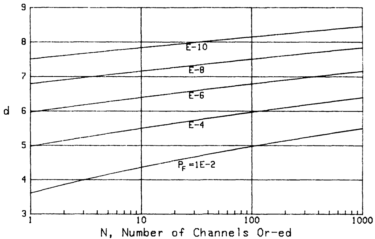
Figure 47. Required d Values for M=4 , P_{c_0}=.5
