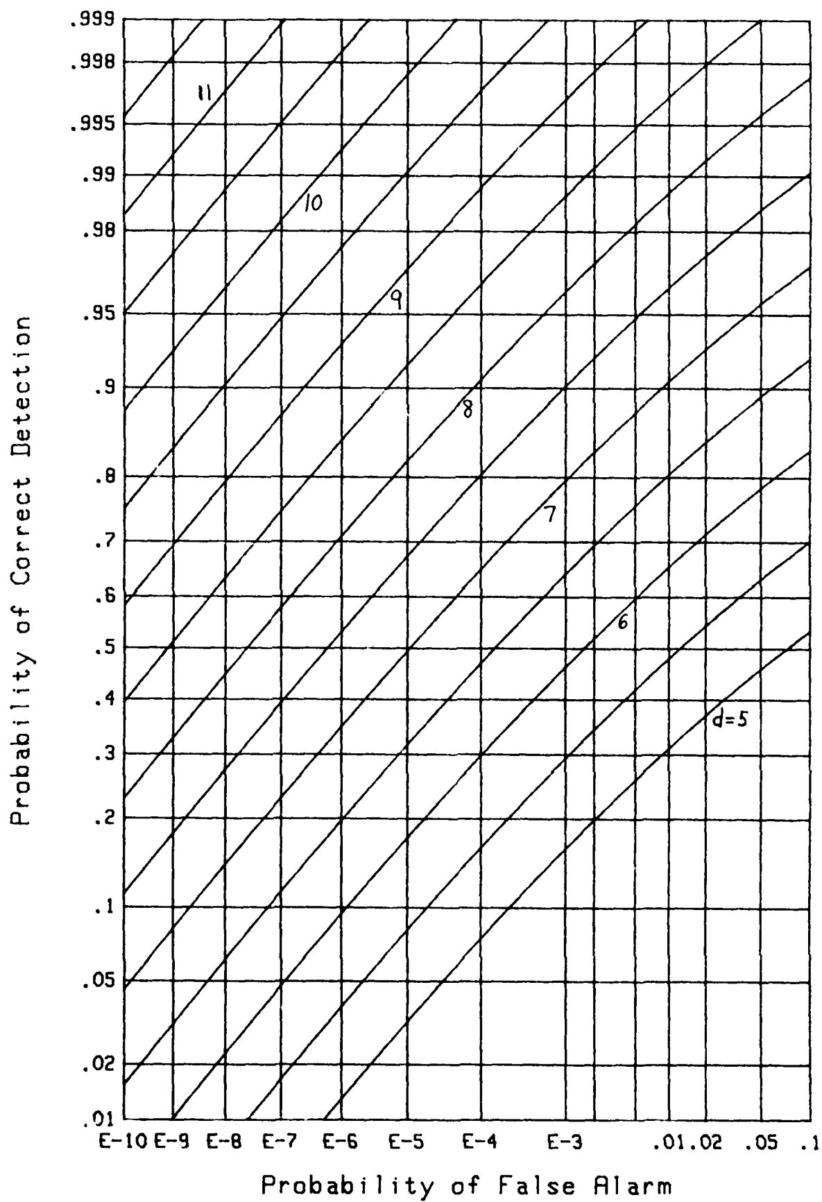
Figure 33. ROC for M=8 , N=100
