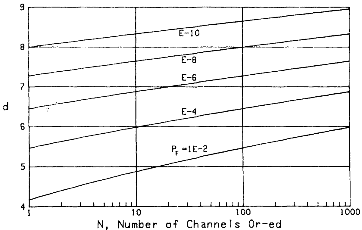
Figure 44. Required d Values for M=1 , P_{cd}=0.9
