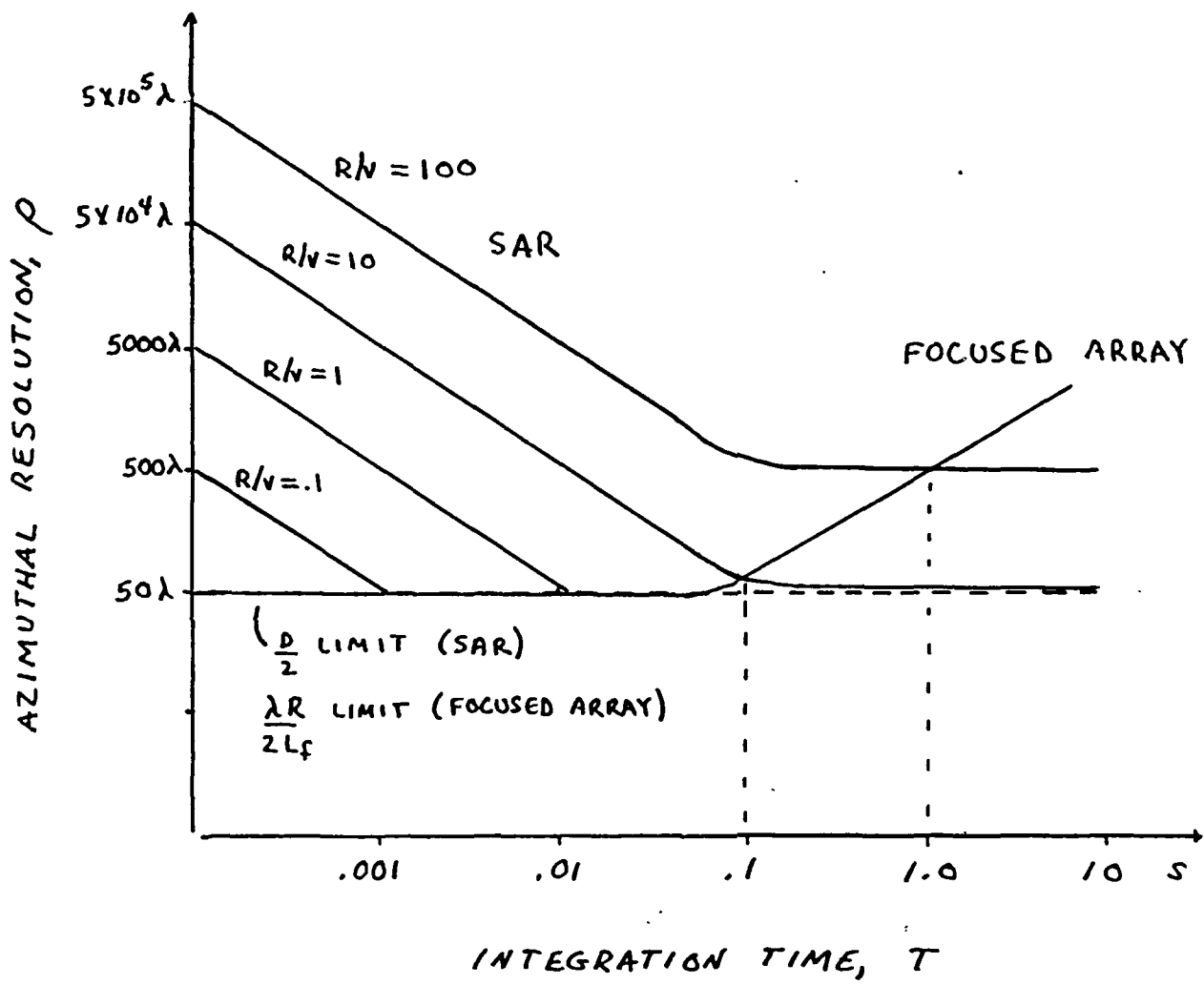
FIGURE 2 - COMPARISON OF EQ. (1) AND (3) SHOWING EQUIVALENCE WHEN (2) IS SATISFIED. ( D = 100 \lambda ; \tau = .15 ; R = 1000 \text{ m} FOR FOCUSED ARRAY; L_f = 10 \text{ m} ).
