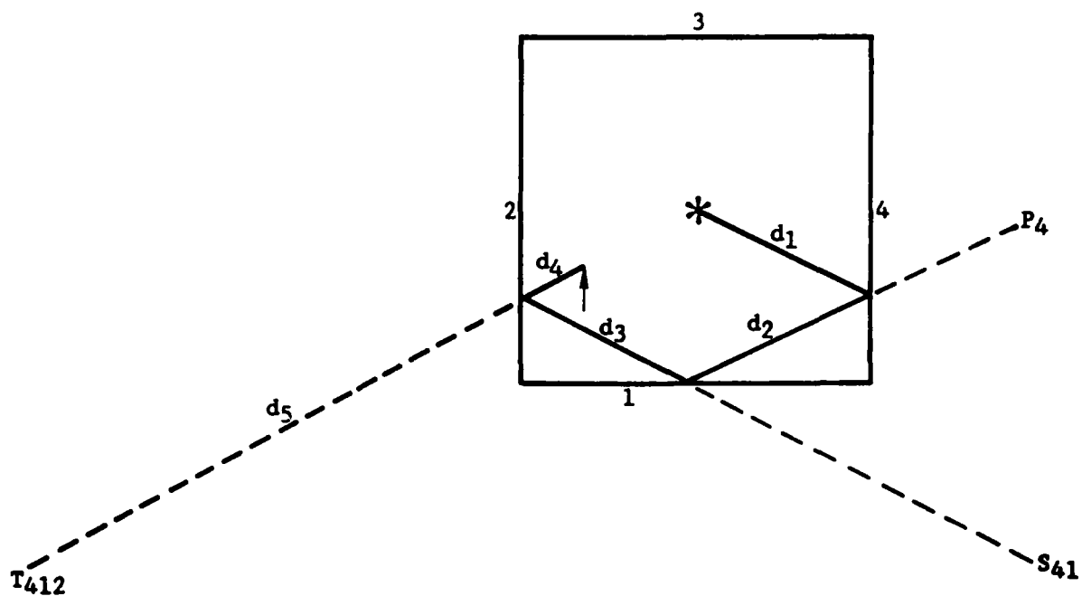
Figure 4. Third order reflection. The distance, d_5 , between the sensor (1) and the tertiary image, T_{412} , is equal to the path of the blast wave, d_4, d_3, d_2, d_1 . (d_5 = d_4 + d_3 + d_2 + d_1)
