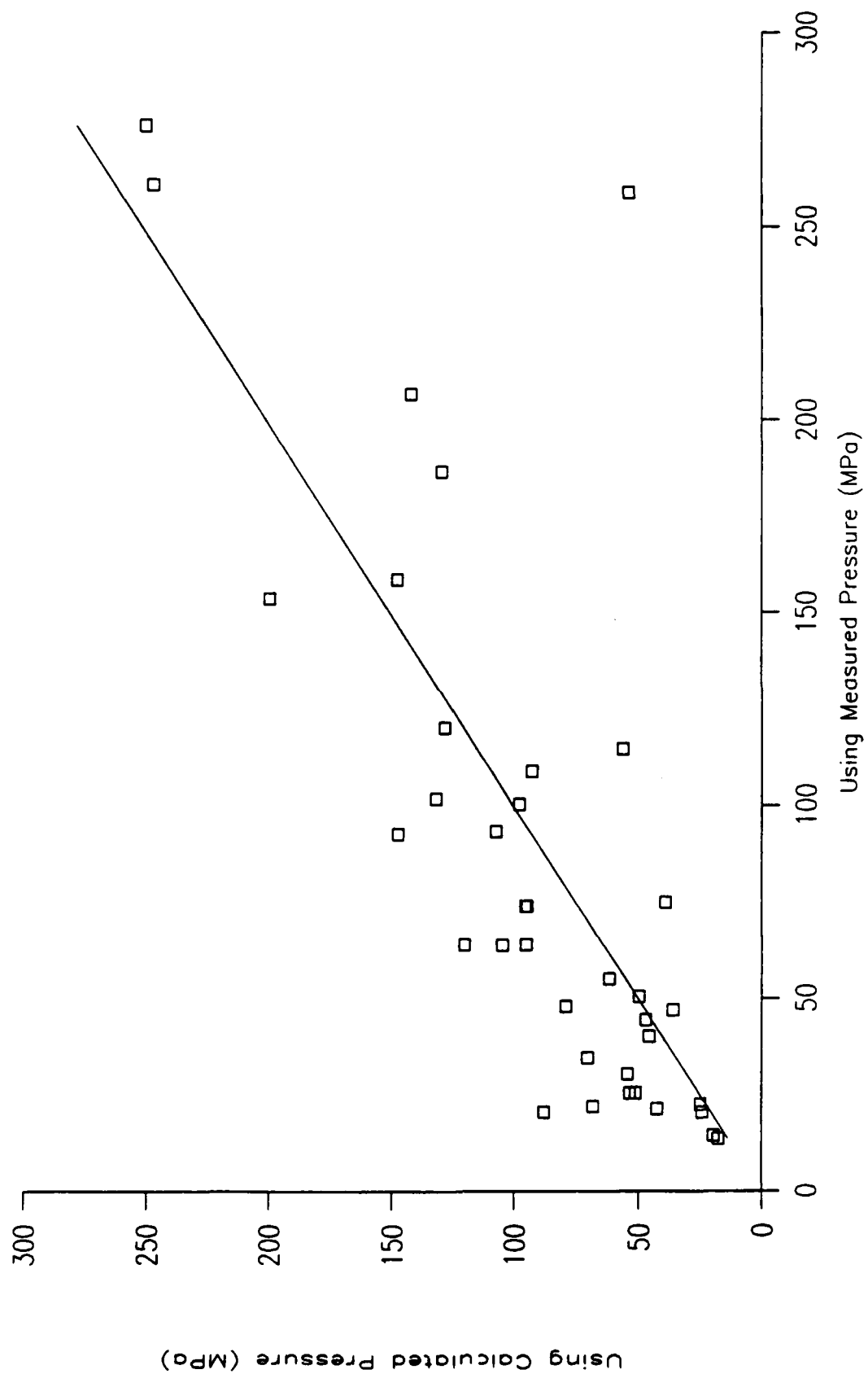
Figure 13. Tympanic stress.
