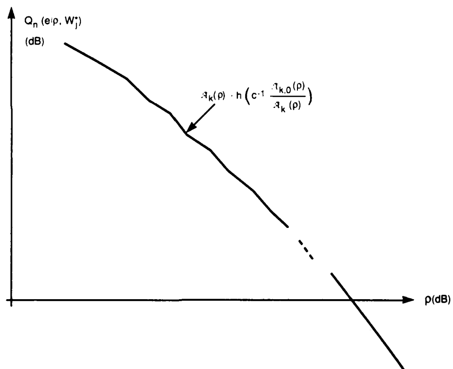
Figure 4-7 Geometric interpretation of the worst-case performance.
