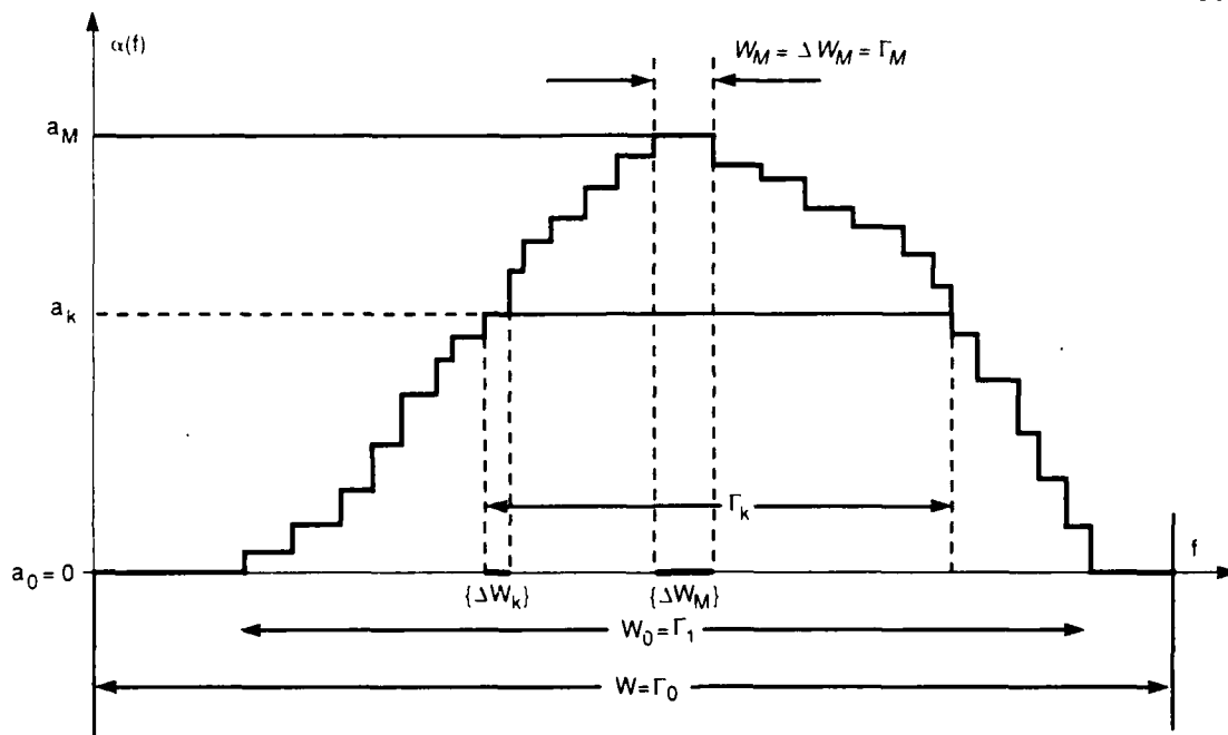
Figure 4-1. Staircase-like discrete distribution.
