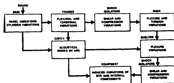
Fig. 6 Paths of Structural Vibration and Airborne Noise into the Equipment Rack.
