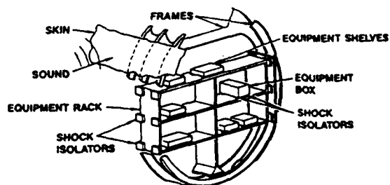
Fig. 5 Forward Equipment Rack Mounted on Vibration Isolators (Without Center Post).
