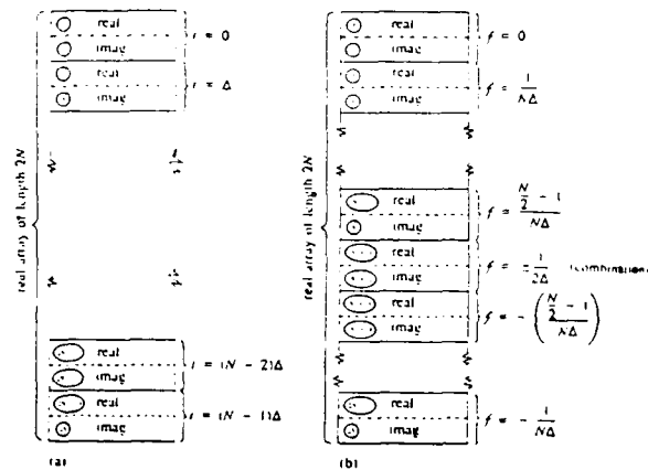
Figure II.1 Storage convention for input/output data array DATA1 (after Press et al. 1986).
