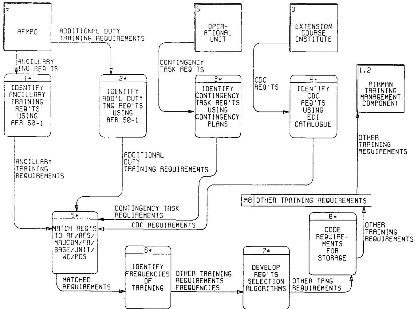
DFD 1.1.5, MANAGE OTHER TRAINING REQUIREMENTS (SPEC. PARA. 3.7.1)
