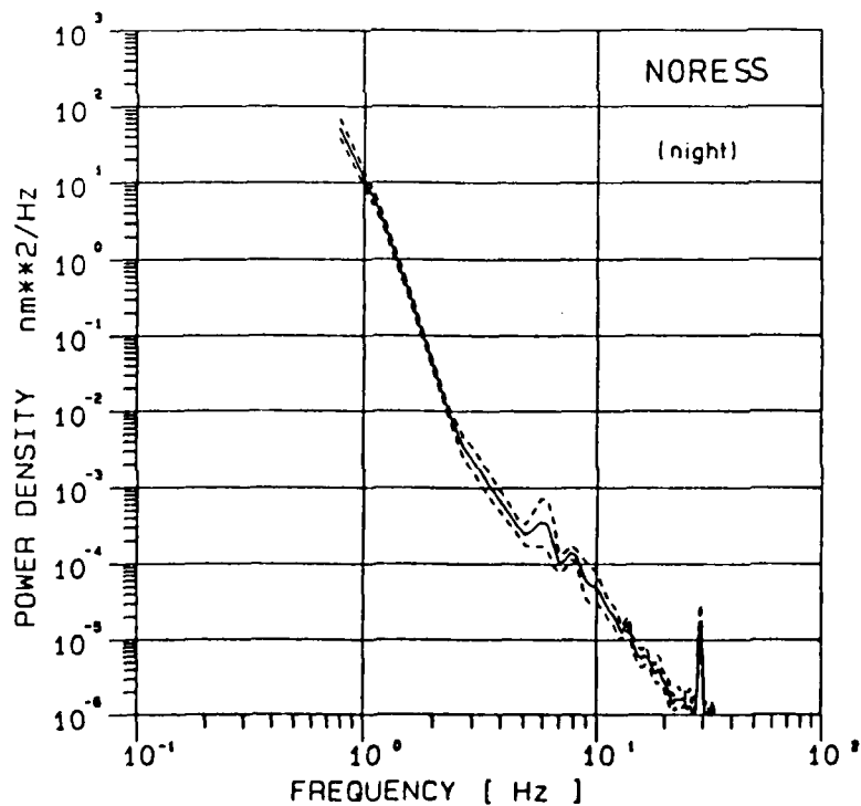
Fig. 4 : Displacement power spectra of noise at NORESS (site C4). For explanation see Fig. 2.
