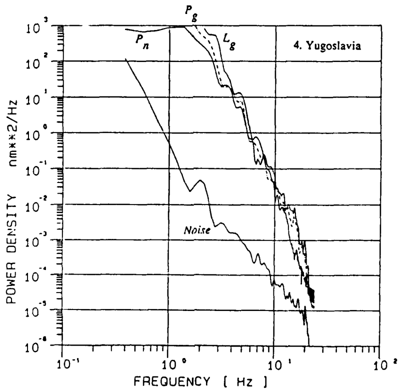
Fig. 31 : Displacement power spectra of events no 3 and no 4 from Table 1.
