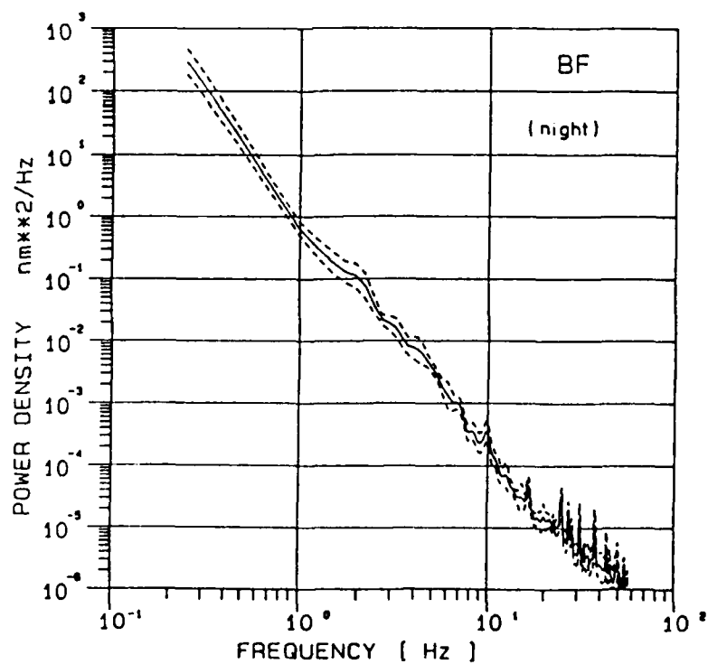
Fig. 2 : Displacement power spectra of noise in the Bavarian Forest (BF) area for day and night. Solid line represents an average of 12 different data samples, dotted lines mean plus/minus one standard deviation
