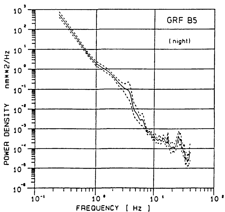
Fig. 3 : Displacement power spectra of noise at the GRF-array (site B5). For explanation see Fig. 2.
