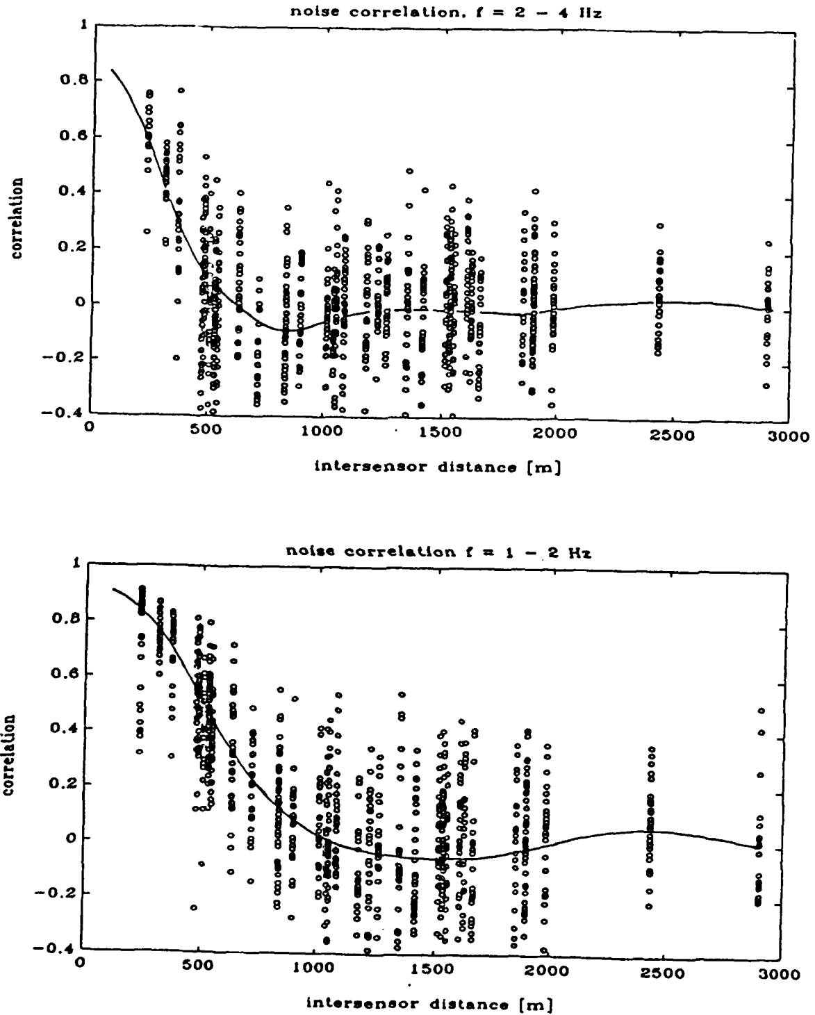
Fig. 7 : Noise correlation values within the test-array. (top : prefilter 2 Hz - 4 Hz, bottom : 1 Hz - 2 Hz passband) The solid lines represent a smoothed average curves.
