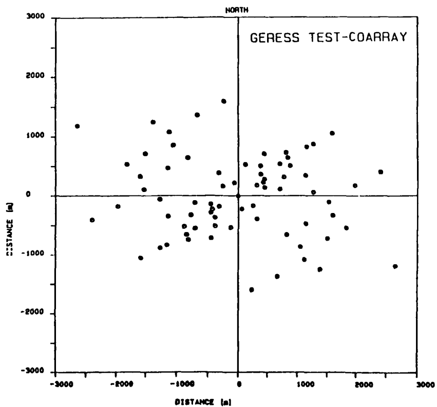
Fig. 5 : Nine-element test-array in the BF-area. Coordinates of central vault: 48.845N, 13.700E. The coarray on the right side shows all interstation distances in vector space.
