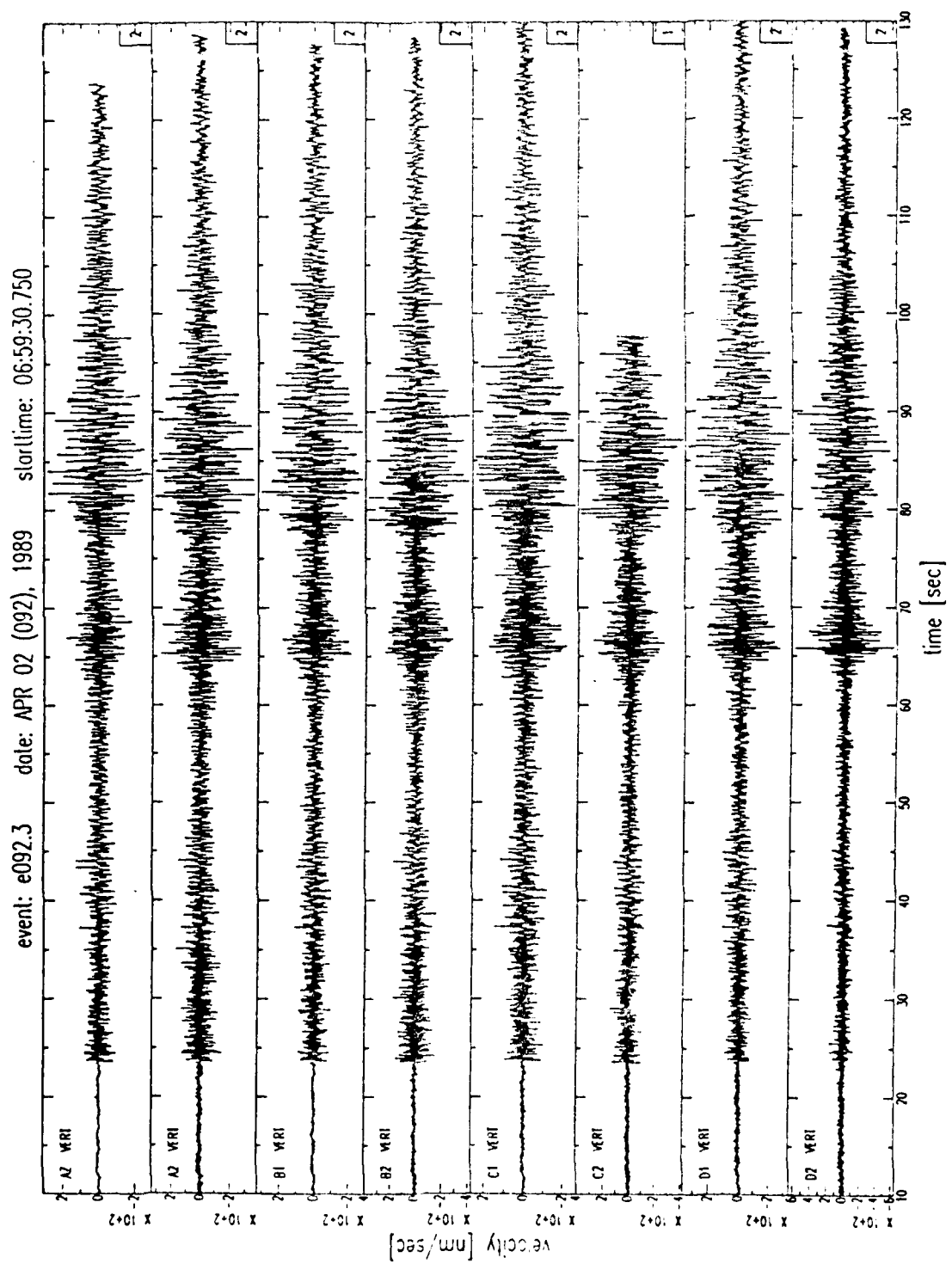
Fig. 28 : Event 7 : Switzerland 01/07/1989 02:29:42.4
