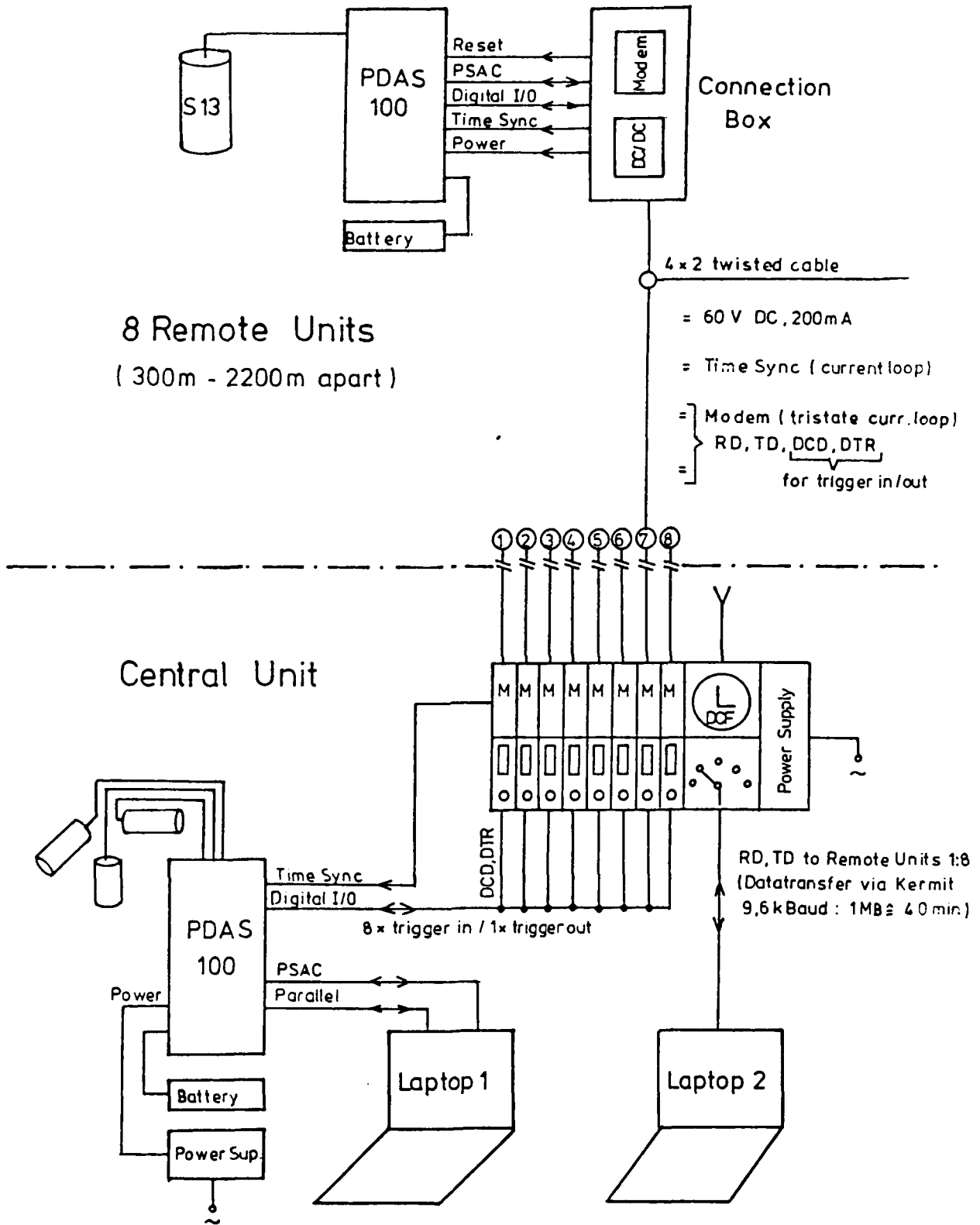
Fig. 15 : Block diagram of GERESS test array
