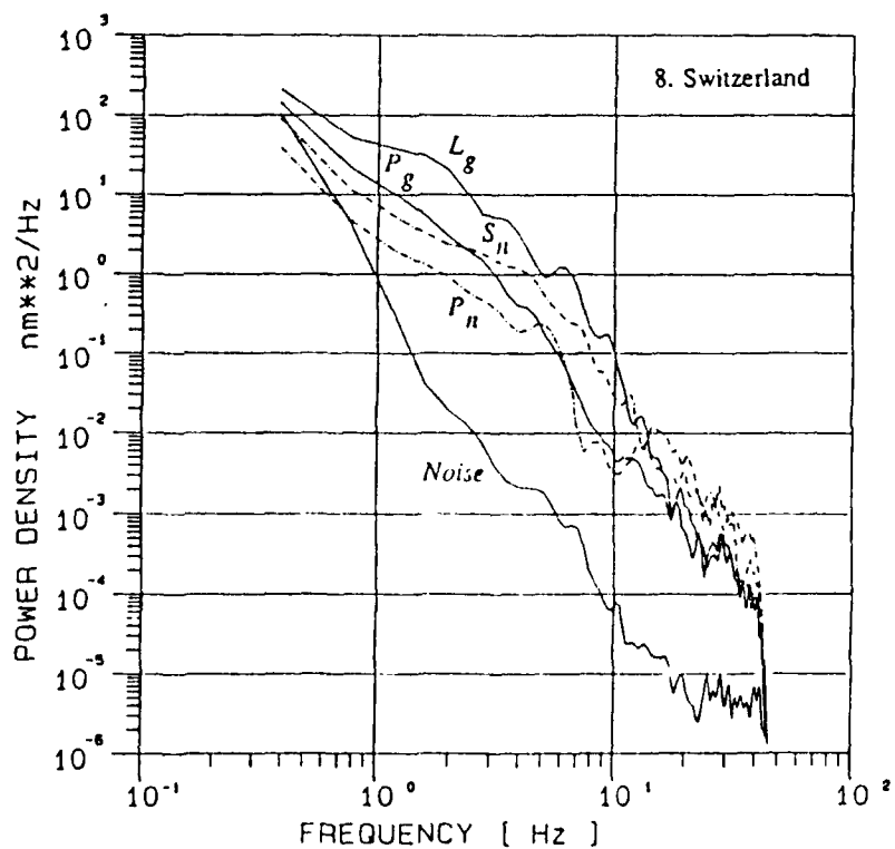
Fig. 30 : Displacement power spectra of events no 1 and no 8 from Table 1.
