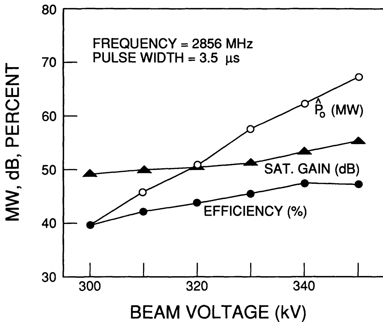
Fig. 2 — Amplification, power and efficiency of a SLAC klystron as a function of voltage
