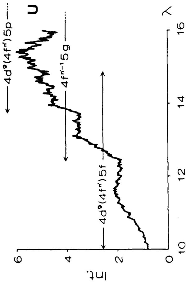
Fig. 6 — Experimental intensity traces from laser-irradiated a) gold, b) bismuth, c) uranium targets with intensity units in 10^{17} eV/sr-Å and wavelength scale in Å. The lower traces are plots of the calculated gA values for: a) the Au 4d^n \rightarrow 4d^{n-1}5f and 4p^64d^n \rightarrow 4p^55d sequences, b) the Bi 4 \rightarrow 5 transition sequences as described in text. In c) the upper states of uranium ion transitions for ions with 4d^{10}4f^n ground state are indicated on horizontal lines (uranium ion sequence U XXXIII to U XLVI). The line extent represents the sequence wavelength range.
