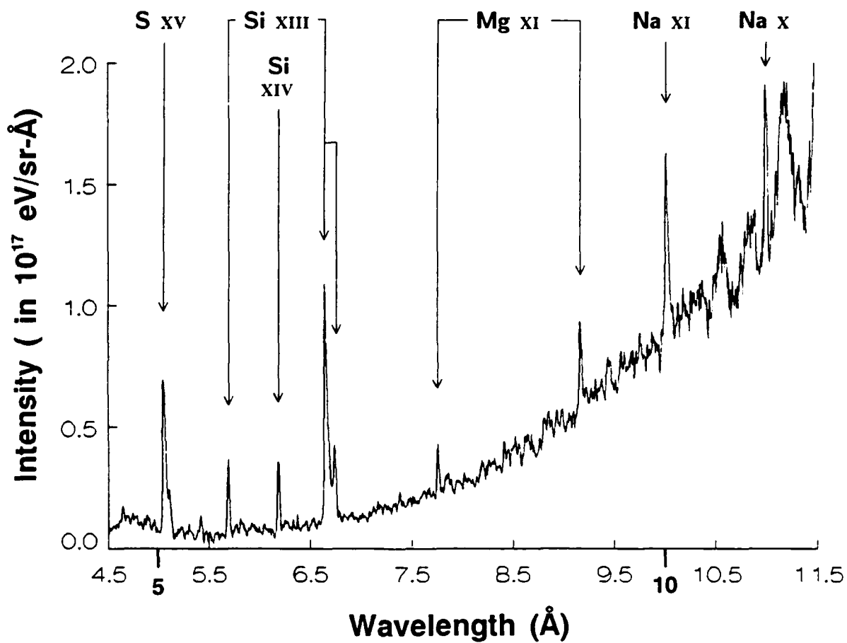
Fig. 3 — Spectral intensity trace from a \text{BaBi}_{0.4}\text{Pb}_{0.6}\text{O}_3 microfragment with impurity lines used for wavelength calibration
