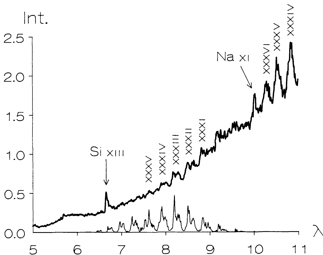
Fig. 5 — Experimental intensity trace from a laser-irradiated \text{BaBi}_4\text{Pb}_6\text{O}_3 compound (intensity in 10^{17} \text{ eV/sr-}\text{\AA} and wavelength in \text{\AA} ). The lower trace is a plot of the calculated gA values for the Ba ion transition sequence with 3d^{n-1}5f and 6f excited states.
