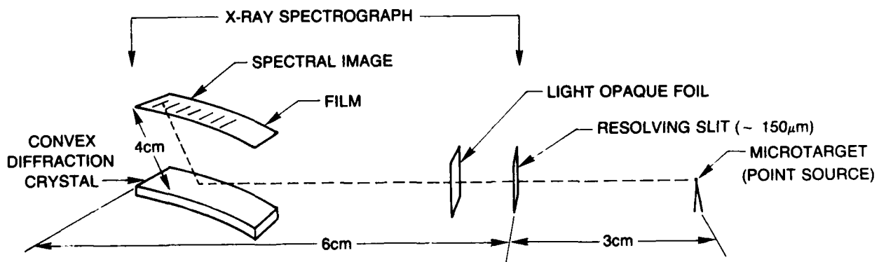
Fig. 2 — Experimental arrangement with typical dimensions
