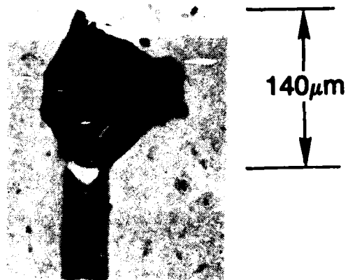
Fig. 1 — Microtarget ( \text{BaBi}_{0.4}\text{Pb}_{0.6}\text{O}_3 ) mounted on a glass stalk
