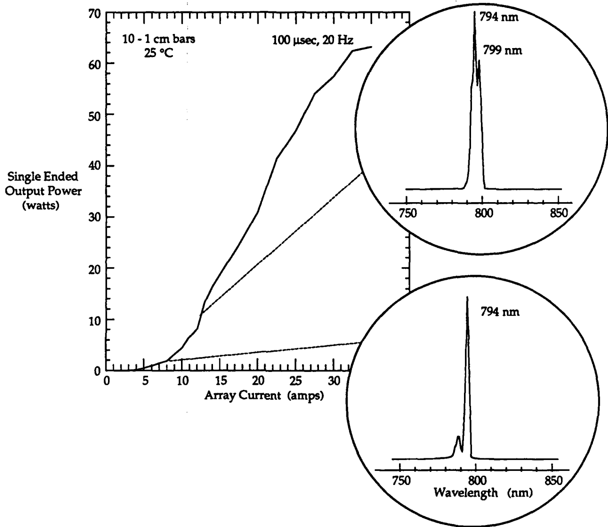
Figure 5. Power versus current relationship and emission spectra of a 2D, 10 bar assembly taken at 100 μsec pulses at 20 Hz.
