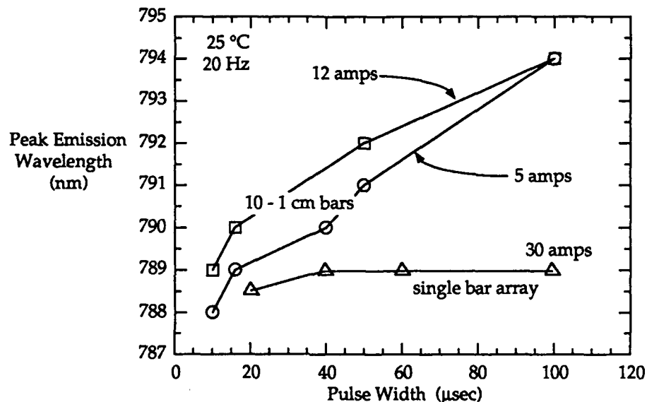
Figure 6. Peak emission wavelength plotted verses pulse width for the same array whose PI curve appears in figure 5. The current level for each set of data is indicated in the figure. For comparison data is included on a linear array assembly fabricated by the new method.
