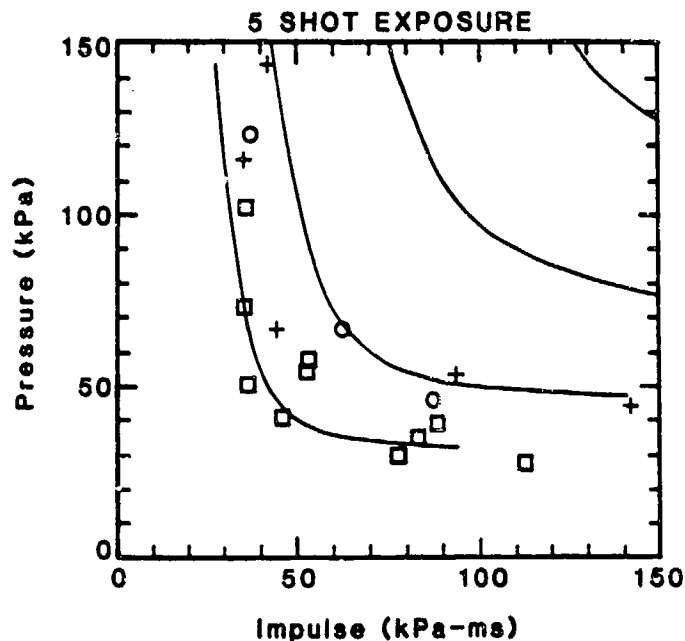
Figure 3. Comparison of generic model predictions with data taken from [7] on observed larynx injury in sheep exposed to 5 shots. Symbols indicate observed injury level: \square , none; \circ , trivial; +, slight; \blacksquare , moderate; \bullet , severe. Curves are equal stress contours based on the generic model for s(1) = 69 kPa, 109 kPa, 188 kPa, 295 kPa and a fatigue factor f = 0.2 .
