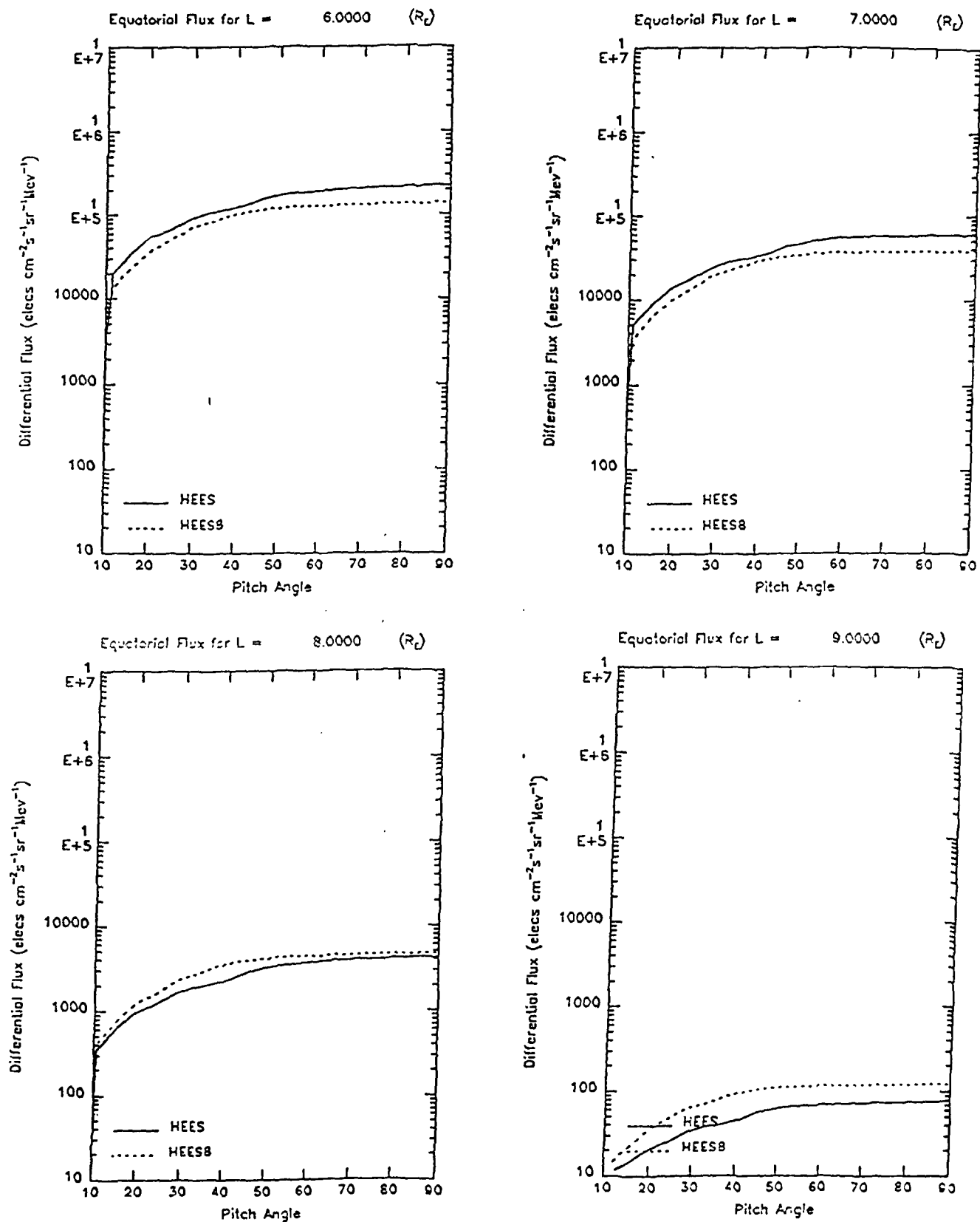
Figure 4c: Unidirectional differential flux vs. pitch angle for electrons with energies between 1.0-1.5 MeV for L=6.0-9.0 R E . The differences are slightly larger than those seen at lower L-shells between HEES (AE6MAX + AEI7HI) and HEES8 (AE8MAX)
