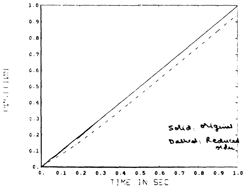
Figure 7. Ramp response
