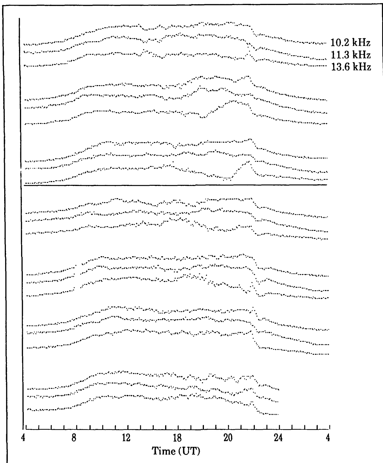
Figure 27. Received Phase, Japan at Cubi Point 01-07 January 1987
