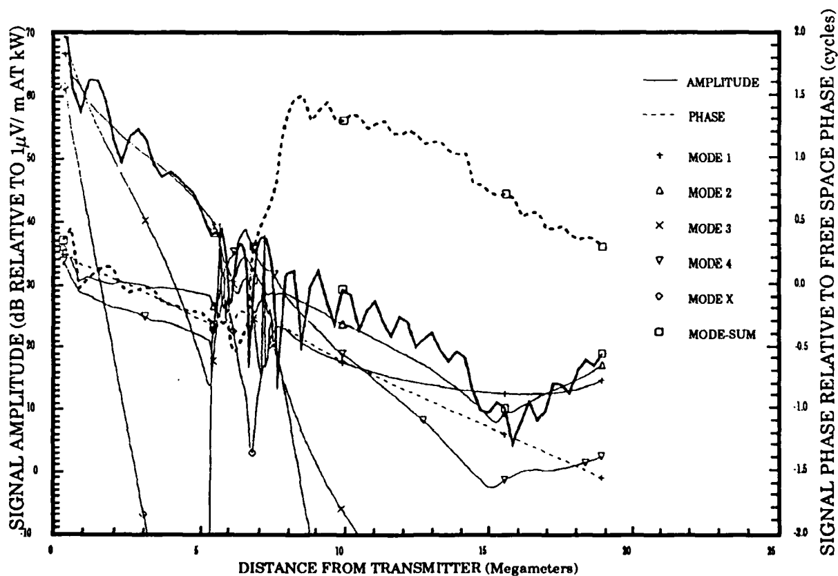
Figure 14(b). North Dakota 13.6 kHz Signal: Night, 224 Degree Radial
