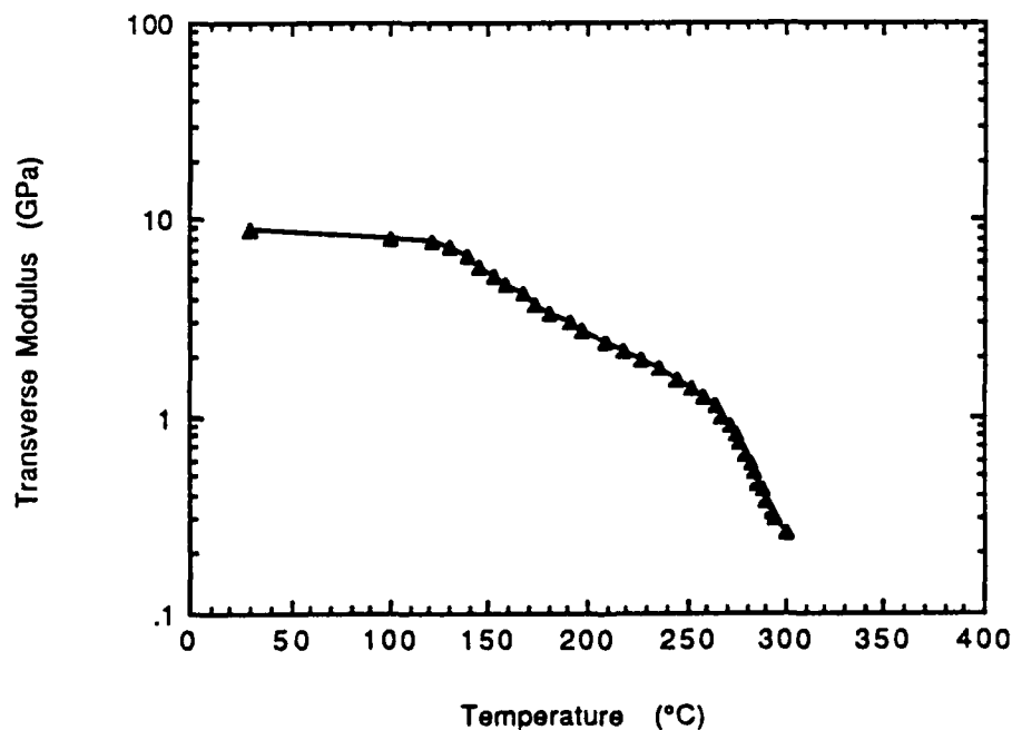
Figure 44. Dynamic Mechanical Measurement of the Temperature-Dependent Transverse Modulus E_T of APC-2 [56].
