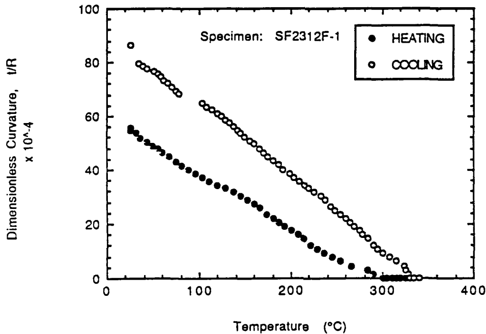
Figure 24. Dimensionless Curvature for a Single SFT Cycle, Phase II, of a [0_3/90_3] Specimen Processed at a Cooling Rate of 74^{\circ}\text{C}/\text{min} (SFT \approx 330^{\circ}\text{C} ).
