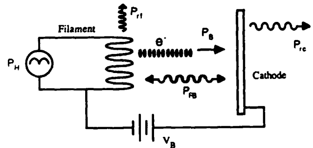
Figure 3: Heating System Model
