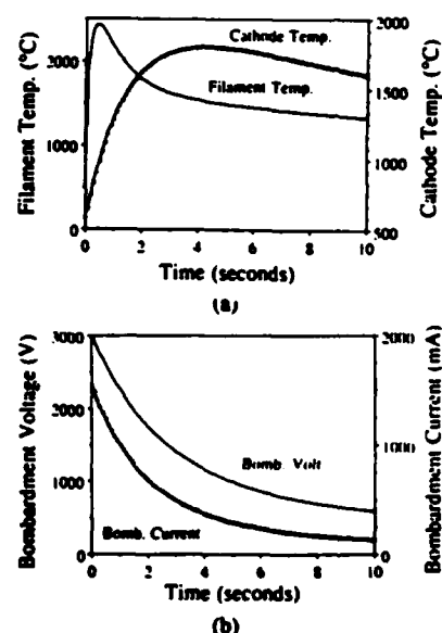
Fig. 4. Simulated 1-in. cathode 120-s cyclic operation for V_{c0} = 3 kV. Other parameters and energy requirements for this case are given in the first line of Table II. (a) Transient filament and cathode temperatures with cathode peak at 1800^\circ\text{C} . (b) Transient bombardment voltage V_B and current I_B . These waveforms repeat every 120 s.
