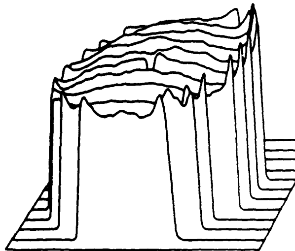
Fig. 5. Lab 2 electron-gun emission profile of the entire beam section. The approximate diameter of the beam at the location of measurement ( z = 4 cm) is 3 cm. Eleven pinhole sweeps were made equally spaced chords
