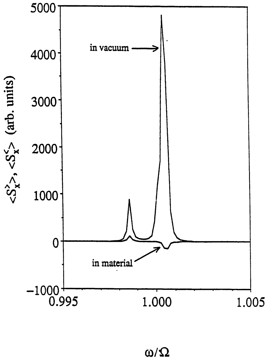
Figure 6.3. Parallel power flows inside and outside the material as functions of frequency on a periodic grating with s = .5c/\Omega . The quantities shown are proportional to \langle S_x^> and \langle S_x^< \rangle . There is no applied field, \theta_0 = 45^\circ , and damping is 1/\Omega\tau = .0001 . The larger, higher frequency peak is due to a surface polariton. The other peak results from a surface resonance that lies within the bulk polariton band.
