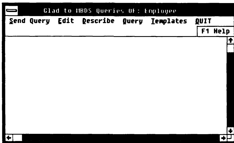
Figure 4.2 QueryWindow
