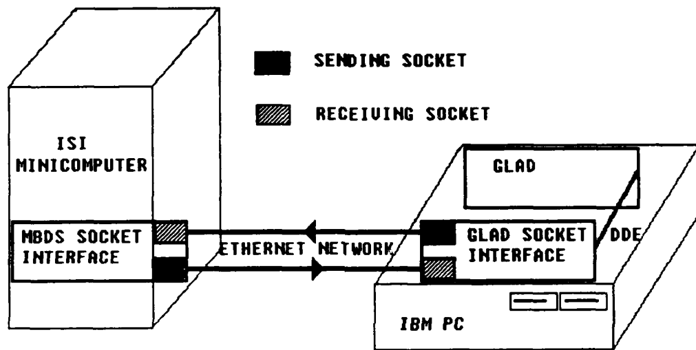
FIGURE 3.5 MBDS/GLAD Interface
