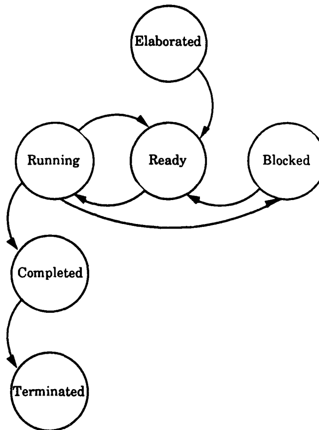
Figure 1. Process states
