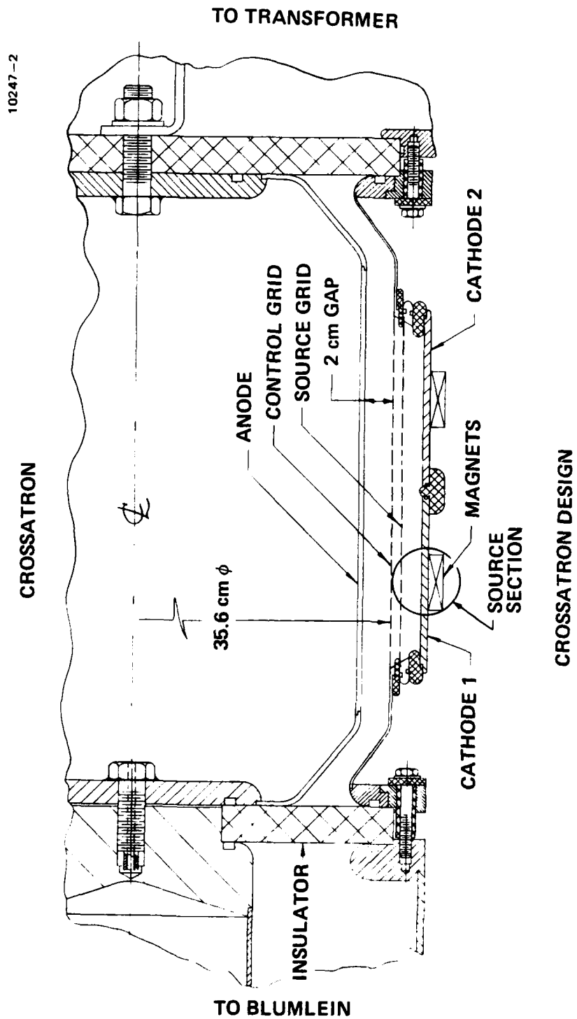
Figure 2. Crossatron design.
