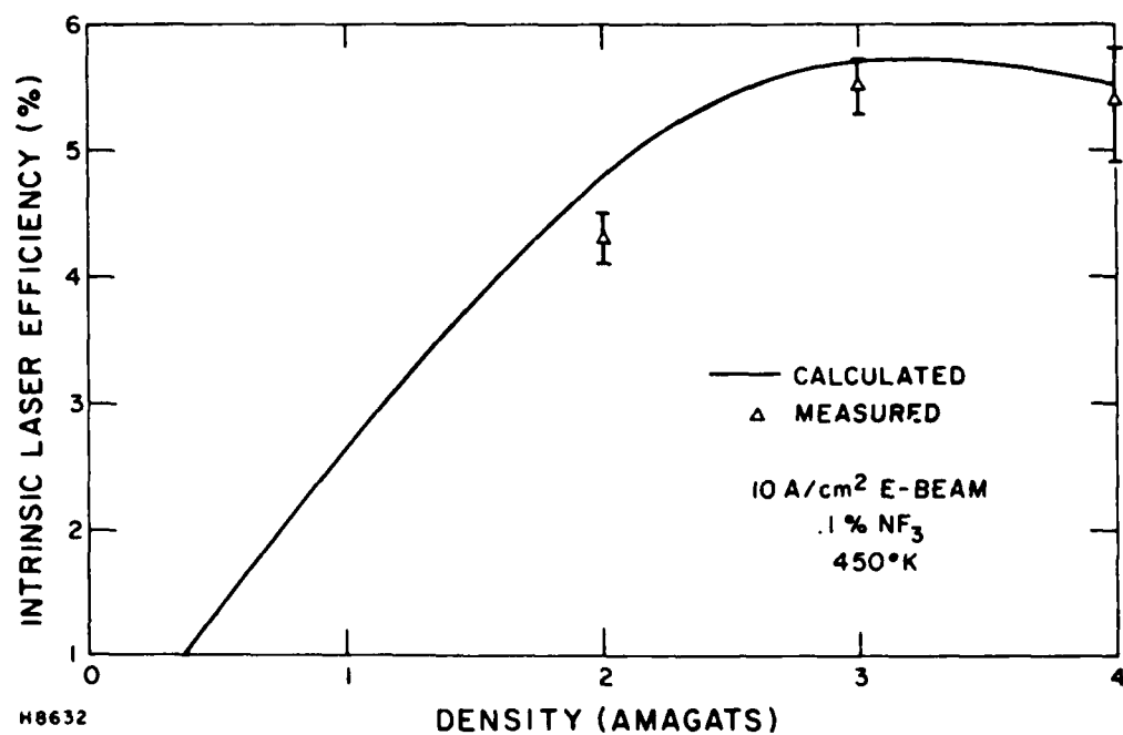
Figure 5. Intrinsic Laser Efficiency vs. Density
