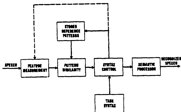
Fig. 8 Block diagram of a speech recognizer incorporating syntax and semantics.
