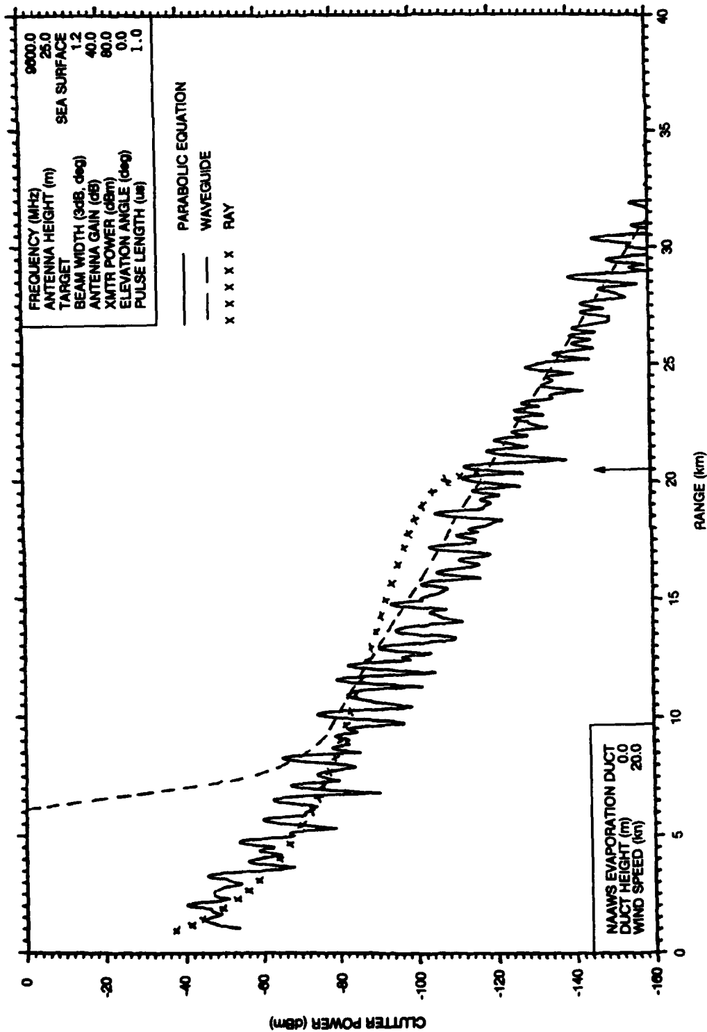
Figure 2. Clutter power vs. range. Comparison between pe, waveguide and ray results. Standard atmosphere, 20 knot wind.
