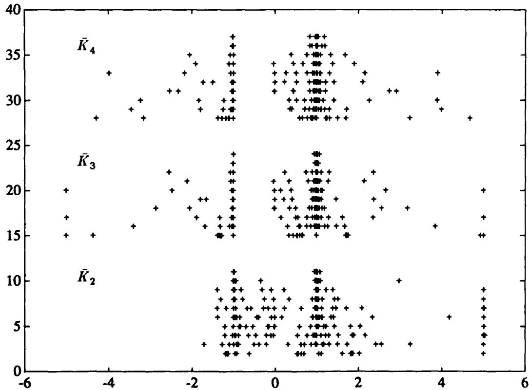
Figure 1: Eigenvalues for \bar{K}_2 , \bar{K}_3 , \bar{K}_4 for problem exp1
