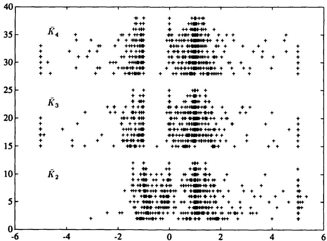
Figure 2: Eigenvalues for \bar{K}_2 , \bar{K}_3 , \bar{K}_4 for problem afiro
