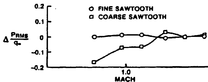
b. Comparison of fine and coarse sawtooth spoilers
