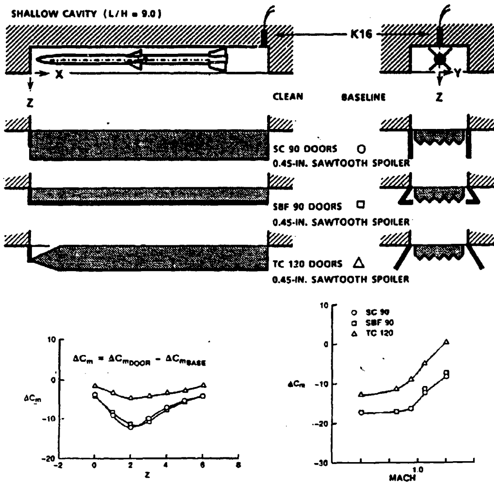
Fig. 23. Difference in pitching moment acting on a store model along a Z-axis translation out of a cavity with a 36 sawtooth spoiler and various styles of doors.
