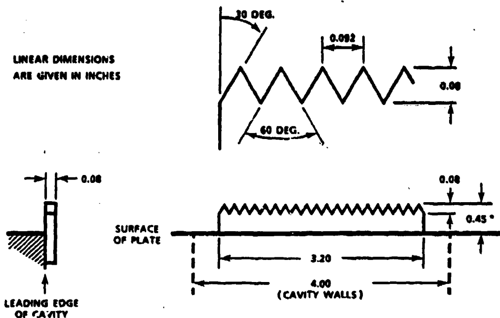
0.45-IN.° SAWTOOTH SPOILER, FINE PITCH
