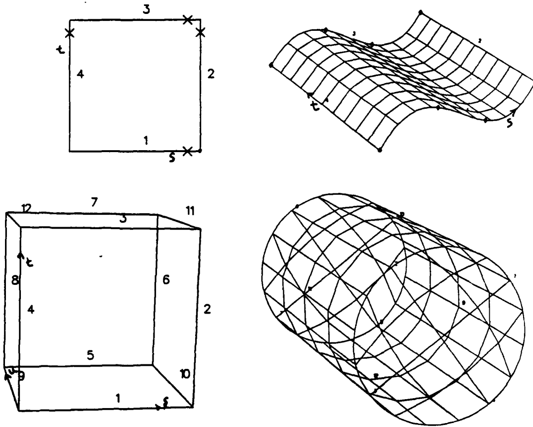
Figure 4: A surface is mapped parametrically into a unit square, and a solid into a unit cube.
